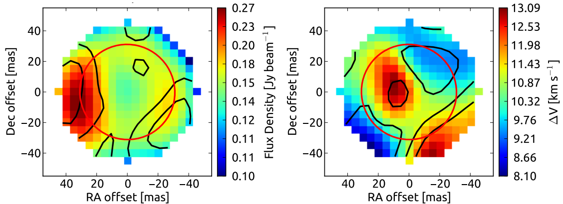
Fig. A.3. Left: intensity map of SiO v = 3, J = 5 - 4 as derived from the pixel-based spectral fit. The contours indicate the fitted rms errors at 2, 3, and 4 mJy beam ^{-1} . Right: FWHM velocity map. The contours indicate the fitted rms errors at levels of 0.26, 0.39, and 0.52 km s ^{-1} .
