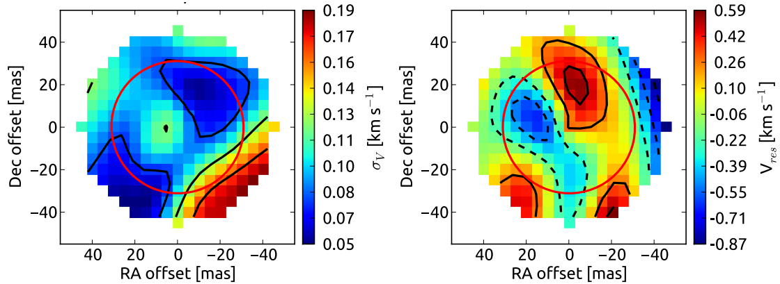
Fig. A.2. Left: velocity error map as derived from the pixel-based spectral fit of the SiO v = 3, J = 5 - 4 line, which we used in the \chi^2 analysis. Right: velocity residual map.
