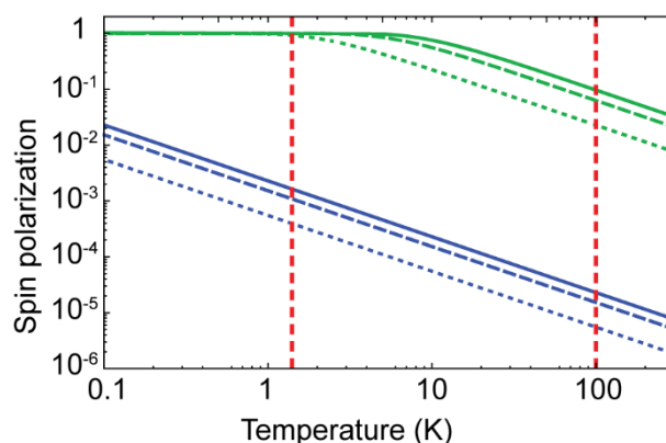
Figure 1: Electron (green) and ^1\text{H} (blue) spin polarization as a function of temperature, for magnetic fields of B_0 = 3.4 T (dotted lines), 9.4 T (dashed lines) and 14.1 T (solid lines). The red vertical lines indicate temperatures of 1.4 K and 100 K.
