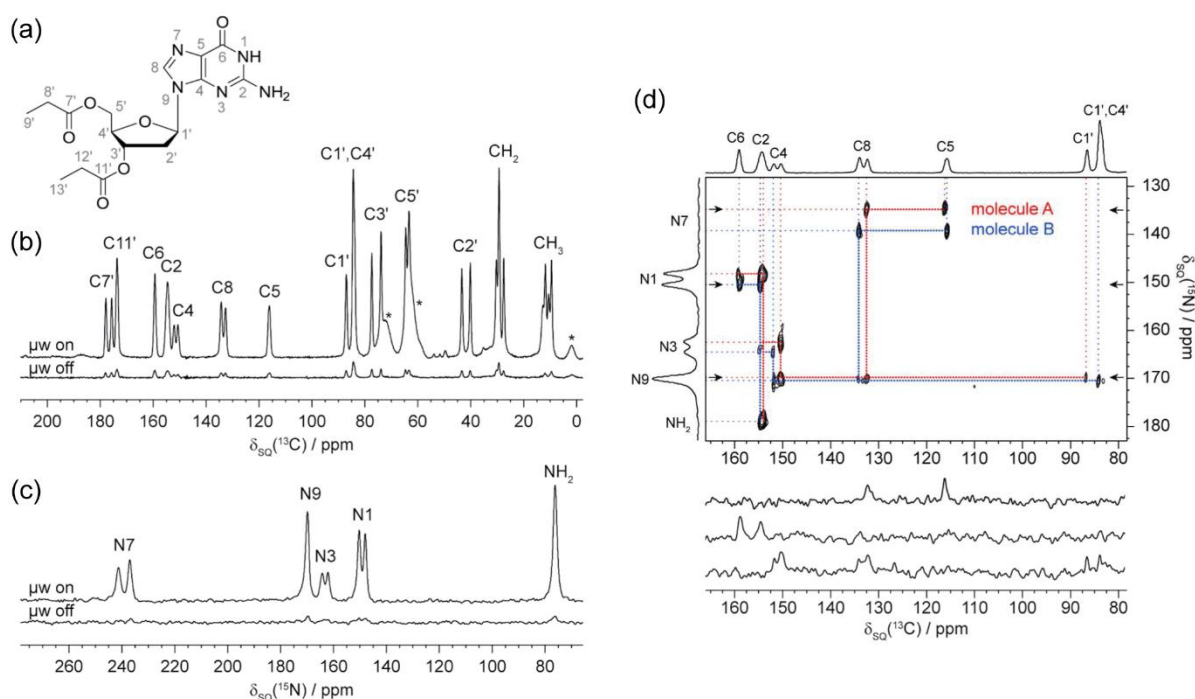
Figure 5: (a) Chemical structure of dG(C3) 2 and ^{13}\text{C} (b) and ^{15}\text{N} (c) CPMAS spectra. Asterisks (*) indicate glycerol and silicon grease (from sample synthesis and preparation). (d) ^{15}\text{N} - ^{13}\text{C} DCP-HETCOR spectrum. ^{15}\text{N} - ^{13}\text{C} polarization transfer was achieved by adiabatic transfer (APHH-CP) with a contact time of 7 ms. The spectrum was recorded in \sim 25 h. The spectral width in the indirect dimension was optimized such that N7 and NH 2 resonances are folded on the respective opposite side of the spectrum. Cross-sections are shown below the spectrum, taken at the positions indicated by arrows. Molecules A and B refer to the two distinct molecules contained in the asymmetric unit cell. The figure and caption are reproduced with permission from ref 86 (Copyright 2015 American Chemical Society).
