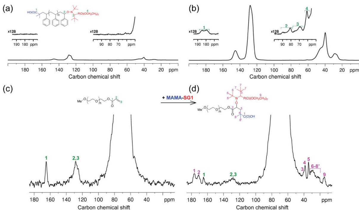
Figure 4: (up) 13 C CPMAS SSNMR spectra of a living PS sample ( M_n = 13\,500\text{ g}\cdot\text{mol}^{-1} ) obtained (a) without or (b) with DNP (at 285 and 105 K, respectively). The sample in (b) was doped with 0.5 wt % bCTbK. In both cases 26 624 scans were used ( \sim 15 h), and intensity scales are identical. (down) 13 C DNP CPMAS SSNMR spectra of an acrylate-terminated PEO sample ( M_n = 35\,000\text{ g}\cdot\text{mol}^{-1} ) obtained before (c) and after (d) the 1,2 intermolecular radical addition with MAMA-SG1. In both cases 0.5 wt % bCTbK and 1600 scans were used ( \sim 13 h). In (d), NMR signals due to both the acrylate PEO and the living PEO samples can be observed, implying that the reaction was not complete. The figure and caption are reproduced from ref 83 (Copyright 2013 American Chemical Society).
