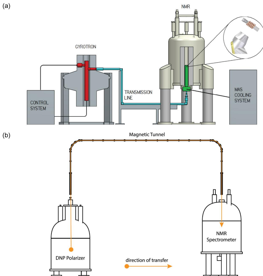
Figure 2: Schematic representation of experimental systems for (a) DNP-MAS NMR consisting of a gyrotron microwave source (gyrotron tube in red), a microwave transmission line (cyan) and an NMR spectrometer equipped with a low-temperature MAS probe (green) and (b) dissolution DNP NMR consisting in a cryostat (DNP polarizer), a transfer line with a magnetic tunnel and an NMR spectrometer equipped with a liquid probe. The figure is reprinted with permission from ref 29 (Copyright 2016 Elsevier) and adapted in part from ref 20 (Copyright 2015 American Institute of Physics).
