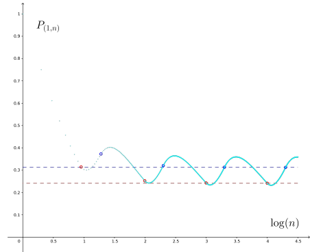
Figure 2: Graph of P_{(1,n)} versus \log(n) , values of P_{(1,\phi(n))} being in red and those of P_{(1,\psi(n))} being in deep blue. Limits \alpha_1 and \beta_1 of these two subsequences are represented by horizontal asymptotes.
