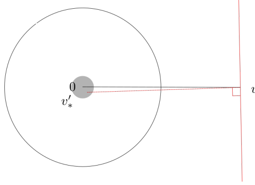
FIGURE 2. The good term: \mathcal{G} corresponds to the integration over the red (plain) line ( \{v' \in \mathbb{R}^d : v' - v \perp w\} ). The grey ball is of radius c_q|v| while the larger ball is of radius |v|/2 .
