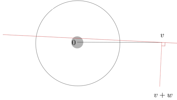
FIGURE 1. The good term: \mathcal{G}(f, f) corresponds to the integration over the red (plain) line (\{v' \in \mathbb{R}^d : v' - v \perp w\}) . The grey ball is of radius c_q|v| while the larger ball is of radius \frac{1}{2}|v| .
