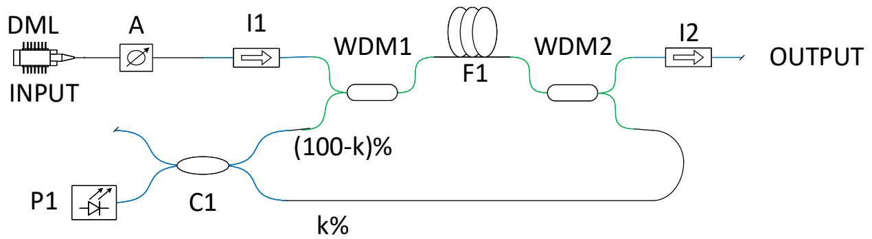
Figure 1. Optical Design of Single Stage Single Pump TDFAs with a Shared Pump Arrangement.
