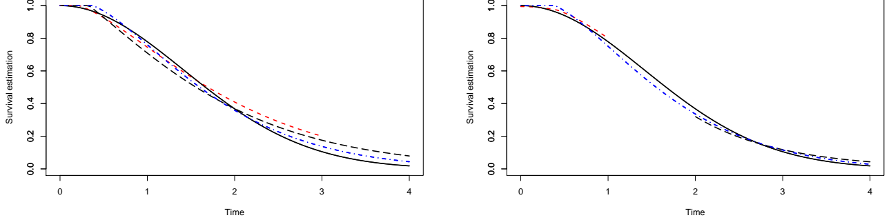
FIGURE 1. True survival curve (black solid line) S_I for Model 1 and Laguerre basis estimators with sample size n = 1000 : \hat{S}_{\hat{m}_L}^{(L)} (red dashed line) built on \text{supp}(L) , \hat{S}_{\hat{m}_U}^{(U)} (black longdashed line) built on \text{supp}(U) and \hat{S}_{\hat{m}} (blue dotdashed line) built on I = [0, 4] on two different scenarios : on the left, scenario 1 with \text{supp}(L) = [0, 3] , \text{supp}(U) = [0, 4] , on the right, scenario 4 with \text{supp}(L) = [0, 1] , \text{supp}(U) = [2, 4] .
