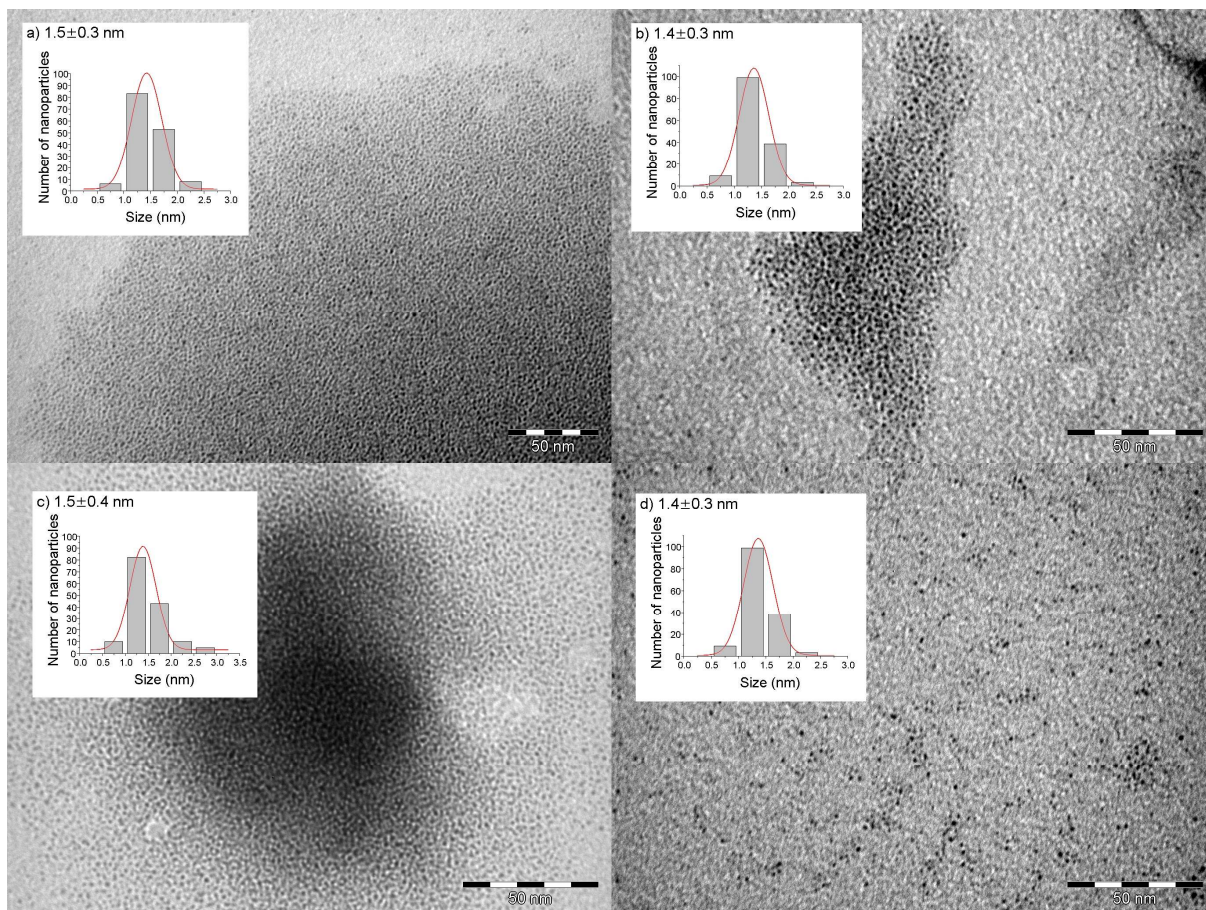
Figure 2. TEM images with the corresponding size histograms of: a) Pt1Ru1 , b) Pt1Ru2 , c) Pt1Ru4 and d) Pt/CO NPs .
