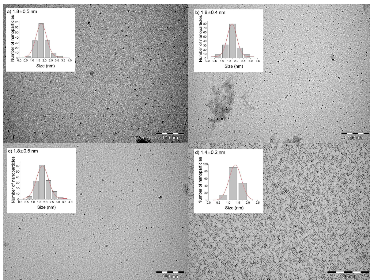
Figure 1. TEM images with the corresponding size histograms of: a) Ru1Pt1 , b) Ru1Pt2 , c) Ru1Pt4 and d) Ru/PPP NPs .
