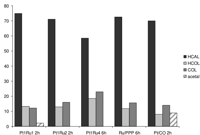
Figure 12. Selectivity in trans -cinnamaldehyde hydrogenation for PtRu series.
