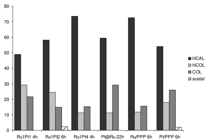
Figure 10. Selectivity in trans -cinnamaldehyde hydrogenation for RuPt series.
