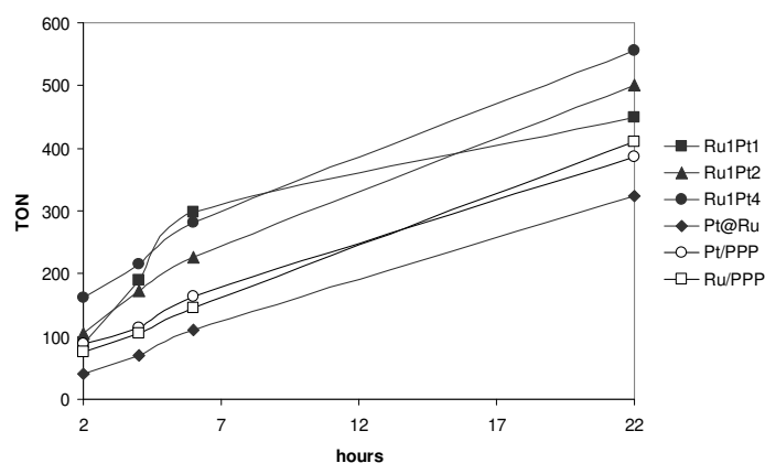
Figure 9. Evolution of TON with time in the CAL hydrogenation using RuPt NPs.
