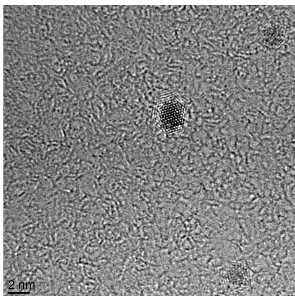
Figure 3. HRTEM image of Ru1Pt2 NPs .
