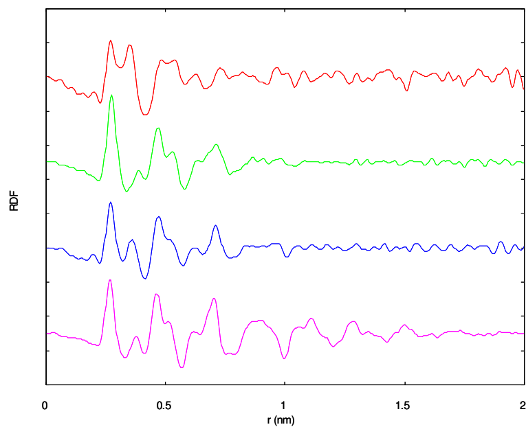
Figure 6. WAXS analysis of bimetallic PtRu NPs (from top to bottom Pt1Ru1 , Pt1Ru2 , Pt1Ru4 and Ru/PPP ).
