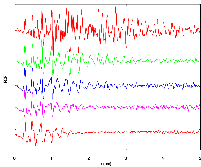
Figure 5. WAXS analysis of bimetallic RuPt NPs (from top to bottom Pt/PPP , Ru1Pt4 , Ru1Pt2 , Ru1Pt1 , Ru/PPP ).
