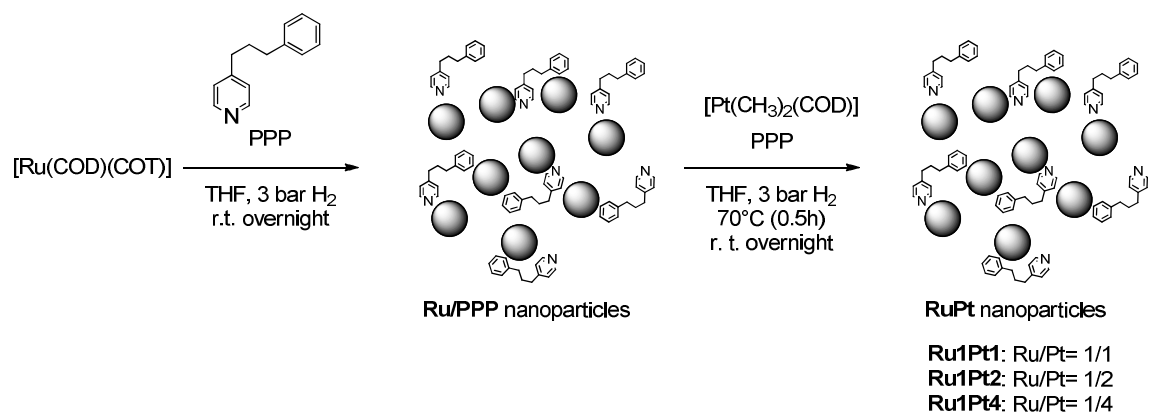
Scheme 1. Synthesis of the RuPt NPs.
