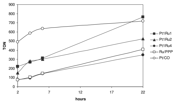
Figure 11. Evolution of TON with time in the CAL hydrogenation using PtRu NPs.
