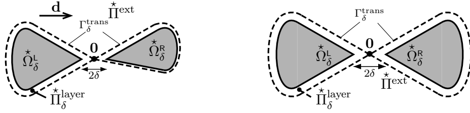
Figure 3: The domain \Pi_\delta^* with the inclusions \Omega_\delta^{LR} (non symmetric and symmetric cases).
