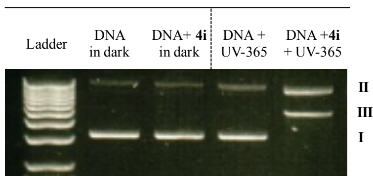
Figure 5. Photochemical cleavage ( \lambda = 365 nm during 1h) of pCDNA3 supercoiled DNA (20 \mu\text{M}/\text{bp} ) by 4i (100 \mu\text{M} ) in TE buffer.
