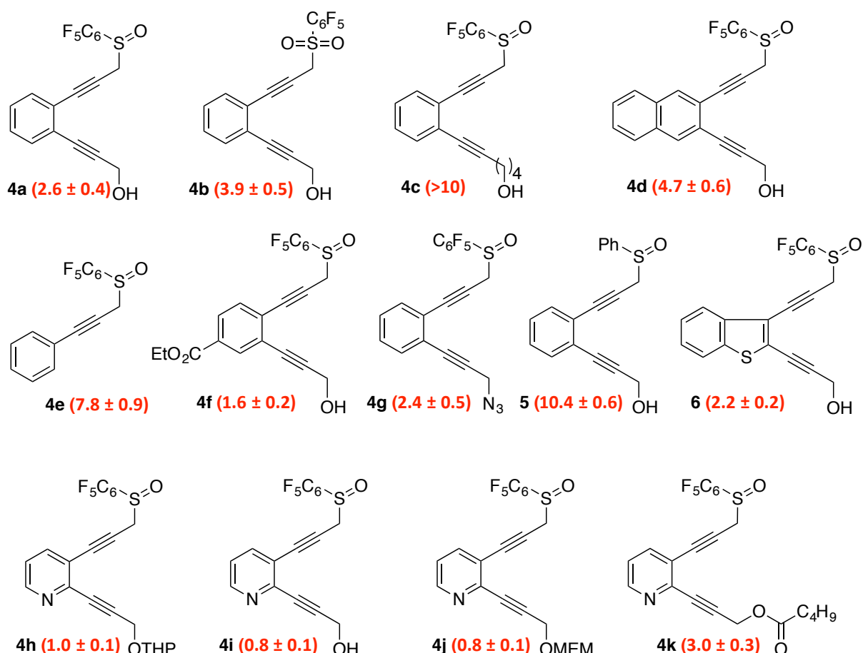
Figure 1 Enediyne Structure and their IC_{50} (in brackets)
