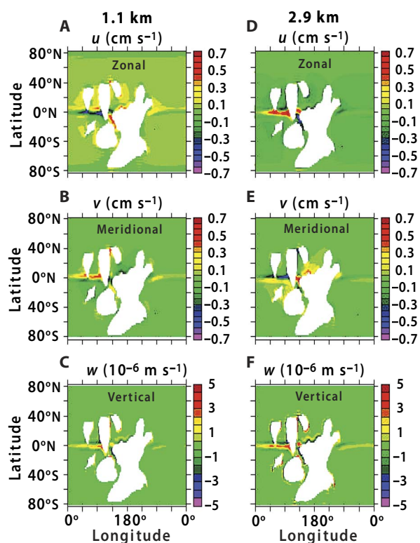
Fig. 21. Snowball Earth ocean circulation, 3D results with Marinoan paleoconcentrations. (A to F) Zonal (A and D), meridional (B and E), and vertical velocity (C and F) fields at depths of -1.1 km (A to C) and -2.9 km (D to F) relative to the ice surface (391). Ice thicknesses are as given in Fig. 20 (A to D). Scale bars are in centimeters per second (A, B, D, and E) and 10^{-6} m s^{-1} (C and F). Positive velocities are westward (A and D), northward (B and E), and upward (C and F). Zonal and meridional velocities change sign with depth, but vertical velocities do not. Strong vertical mixing (C and F) in the zone where cryoconite flushing occurs (Fig. 18B) expedites abyssal sedimentation of finely suspended material. Zonal shallow jets (A) direct flushed cryoconite toward western or eastern ocean margins, in response to excess geothermal input (as in Fig. 20C) from the northern hemisphere.
