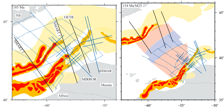
Figure 10. Plate kinematic reconstruction after Seton et al. [2012] of the northern central Atlantic. Magnetic anomalies are marked in two colors (red and orange) depending on its amplitude; extent of the salt basins in yellow. Wide-angle seismic profiles located along the present-day African continent are shown by blue lines and those on the American margin by green lines. Light red shaded region shows the extent of the zone with high lower crustal velocities and the light blue shaded region the extent of thin oceanic crust. NS = Nova Scotia.
