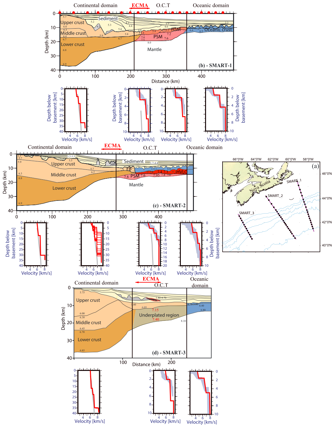
Figure 3. (a) Location of the wide-angle seismic profiles acquired during the SMART project on the regional bathymetry and topography map [Maruyama et al., 1999; Ryan et al., 2009]. (b) Crustal structure modified from the SMART-1 profile [Funk et al., 2004], (c) SMART-2 [Wu et al., 2006], and (d) SMART-3 [Louden et al., 2010]. PSM = partially serpentinized mantle, HSM = highly serpentinized mantle HVLC = high-velocity lower crust, and FB = fault blocks. Numbers represent seismic layer velocities (km/s). Graphs located underneath the profiles represent 1-D velocity-depth profiles extracted from the original velocity models below the top of the basement (vz profiles) from the domain underneath which they are situated. Red lines represents mean vz profiles, the blue shaded area bounds a compilation of velocity profiles of typical Atlantic oceanic crust [White et al., 1992], and bold gray profiles correspond to mean velocity profiles of thinned continental crust [Christensen and Mooney, 1995].
