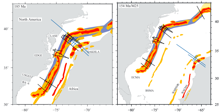
Figure 6. Plate kinematic reconstruction of the northern central Atlantic (poles from Seton et al. [2012]). Magnetic anomalies are marked in two colors (red and orange) depending on its amplitude, the extent of the underplate is shown in blue, and the extent of the salt basins is indicated in yellow. Wide-angle seismic profiles located along present day African continent are shown by blue lines and those on the American margin by green lines.
