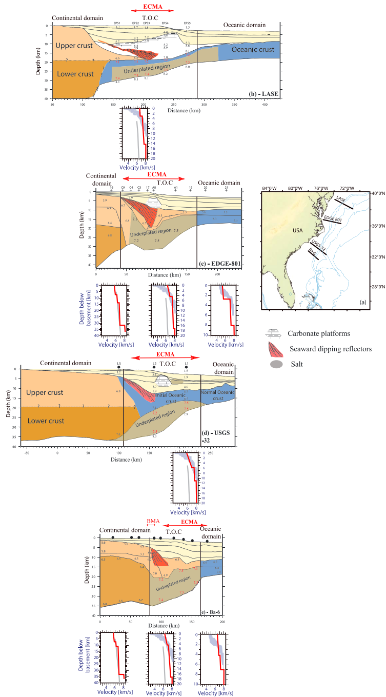
Figure 4. (a) Location of the wide-angle seismic profiles acquired along the U.S. continental margin on the regional bathymetry and topography map [Maruyama et al. , 1999; Ryan et al. , 2009]. Crustal structure modified after (b) LASE profile [LASE Study Group, 1986], (c) EDGE-801 [Holbrook et al. , 1994a], (d) USGS-32 [Tréhu et al. , 1989], and (e) Ba-6 [Austin et al. , 1990; Holbrook et al. , 1994b]. Numbers represent seismic layer velocities (km/s). (For comparisons see also Sahabi et al. [2004] and Labails [2007]). Graphs located underneath the profiles represent 1-D v z profiles extracted from the original velocity models below the top of the basement from the domain underneath which they are situated. Red lines represent the mean v z profiles, the blue shaded area bounds a compilation of velocity profiles for typical Atlantic oceanic crust [White et al. , 1992], and the bold gray profiles correspond to mean velocity profiles for thinned continental crust [Christensen and Mooney, 1995].
