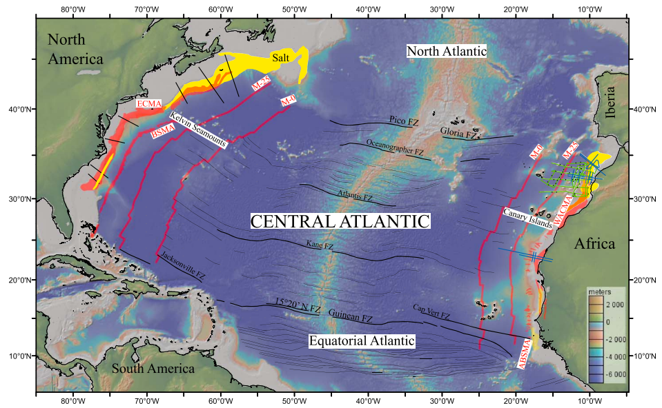
Figure 1. Overview of the central Atlantic Ocean, located between the Pico and Gloria fracture zones to the north and the 15°20'N, and the Guinea fracture zones to the south (thick black lines), bathymetry and topography from [Ryan et al. , 2009]. Major magnetic anomalies ECMA-East Coast, WACMA-West African Coast, BSMA-Blake Spur, ABSMA-African Blake Spur, M25, and M0 are shown in red from Klitgord and Schouten [1986], Sahabi et al. [2004], and Labails et al. [2010]. The position of the salt (light yellow) is taken from Sahabi et al. [2004], Davison [2005], Tari et al. [2012], and the location of the seismic profiles discussed in this study are shown as follows: In blue, wide-angle seismic profiles acquired during the Sismar, DAKHLA, and Mirror cruises [Contrucci et al. , 2004b; Klingelhoefer et al. , 2009; Biari et al. , 2015]. Black dots and green profiles are the positions of sonobuoys and MCS profiles from Holik et al. [1991]. Black lines along the North American margin, represent wide-angle seismic profiles of the SMART-1, -2, and -3 [Funck et al. , 2004; Wu et al. , 2006; Loudon et al. , 2010], LASE, EDGE-801, USGS-32, and BAa-6 [LASE Study Group, 1986; Tréhu et al. , 1989; Austin et al. , 1990; Holbrook et al. , 1994a, 1994b; Lizarralde et al. , 1994; Lizarralde and Holbrook, 1997] going from north to south.
