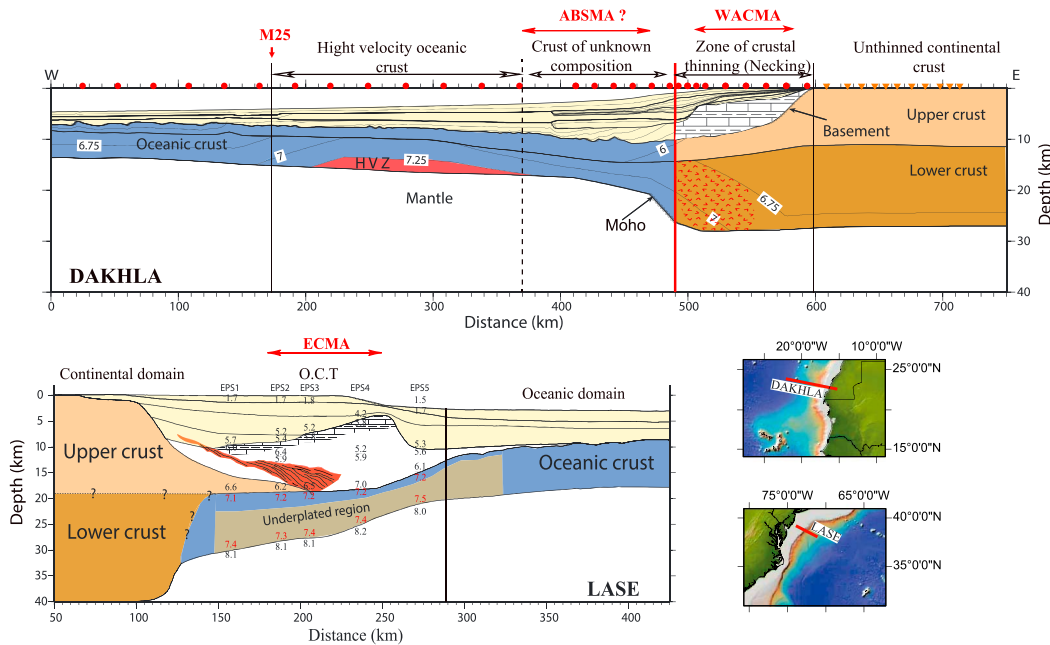
Figure 7. Interpreted depth sections along the conjugate DAKHLA [Klingelhoefer et al., 2009] and LASE [LASE Study Group, 1986] profiles. HVZ = high-velocity zone (mixture of lower crustal material with upper mantle peridotites), numbers represent seismic layer velocities (km/s). Location of the wide-angle seismic profiles acquired during the DAKHLA and LASE surveys on the regional bathymetry and topography map [Ryan et al., 2009].
