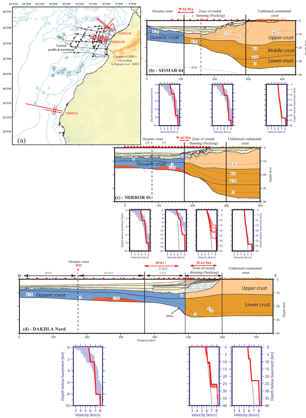
Figure 5. (a) Location of the wide-angle seismic profiles acquired along the Northwest-African margin on the regional bathymetry and topography map [Maruyama et al. , 1999; Ryan et al. , 2009]. Crustal structure modified after (b) SISMAR-4 [Conucci et al. , 2004b], (c) MIRROR-1 [Biari et al. , 2015], and (d) DAKHLA Nord profiles [Klingelhoefer et al. , 2009]. HVOC = high-velocity oceanic crust, CUC = crust of unknown composition, and NOC = normal oceanic crust. Numbers represent seismic layer velocities in km/s. Graphs located underneath the profiles represent 1-D v_z profiles extracted from the original velocity models below the top of the basement, from the domain where they are situated. Red lines represent mean v_z profiles, the blue shaded area bounds a compilation of velocity profiles of typical Atlantic oceanic crust [White et al. , 1992], and bold dark gray profiles correspond to mean velocity profiles for thinned continental crust [Christensen and Mooney, 1995].
