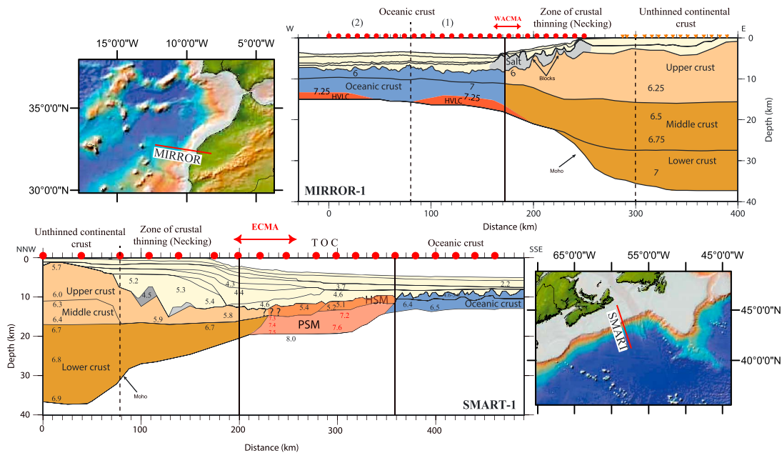
Figure 11. Interpreted depth sections along the conjugate SMART-1 [Funck et al., 2004] and MIRROR-1 [Biari et al., 2015] profiles. PSM = partially serpentinized mantle, HSM = highly serpentinized mantle, and HVLC = high-velocity lower crust. Numbers represent seismic layer velocities (km/s). Location of the wide-angle seismic profiles acquired during MIRROR and SMART surveys on the regional bathymetry and topography map [Ryan et al., 2009].
