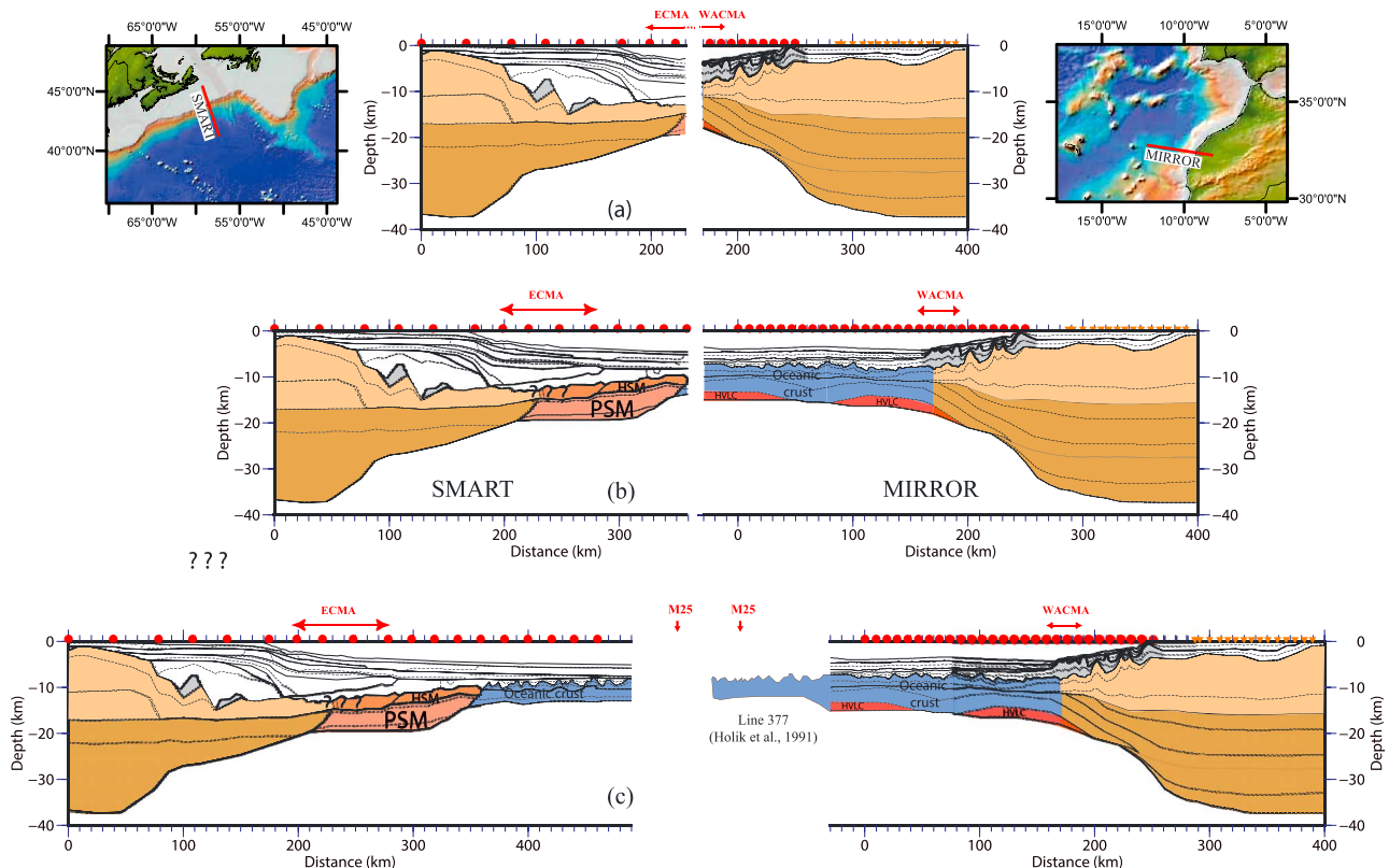
Figure 13. Reconstruction of the Nova-Scotia-Moroccan margin pair. (a) After initial extension, (b) asymmetric seafloor spreading, with exhumation to the west and magmatic accretion to the east, and (c) accretion of thin magmatic oceanic crust.
