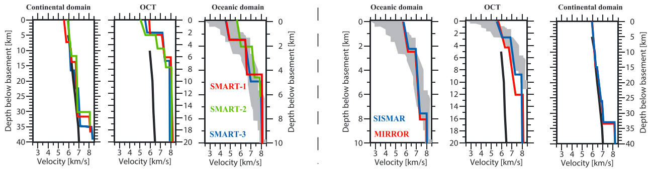
Figure 12. Comparison of vz profiles in the continental, OCT, and oceanic domains between the SMART profiles, SISMAR, and MIRROR profiles. Colored lines represent mean vz profiles, the gray shaded area bounds a compilation of vz profiles for typical Atlantic oceanic crust [White et al., 1992], and the bold black profiles correspond to mean vz profiles for thinned continental crust [Christensen and Mooney, 1995].
