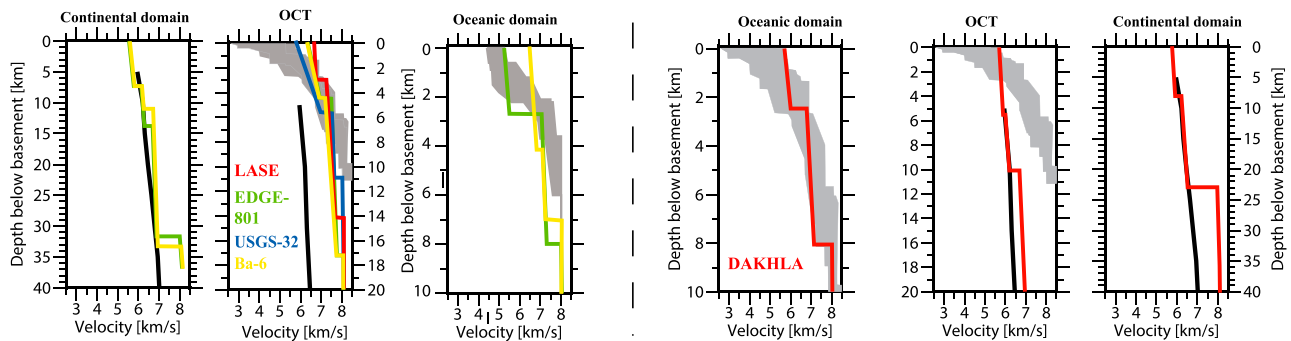
Figure 8. Comparison of v_z profiles underneath the basement in the continental, OCT, and oceanic domains between the U.S. profiles and the DAKHLA profile. Colored lines represent mean v_z profiles, the gray area bounds a compilation of v_z profiles for typical Atlantic oceanic crust [White et al., 1992], and the bold black lines correspond to mean v_z profiles for thinned continental crust [Christensen and Mooney, 1995].
