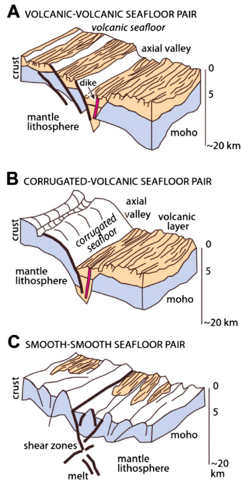
Figure 14. Lithosphere-scale sketches of the axial region for three proposed modes of magma-poor ultraslow spreading, shown in order of decreasing melt supply. Modes A (volcanic-volcanic) and B (corrugated-volcanic) also develop at faster spreading sections of the Mid-Atlantic Ridge and in more magmatically robust regions of ultraslow ridges. Mode C (smooth-smooth or smooth-volcanic), with little to no axial volcanism, appears specific to magma-poor ultraslow ridges [after Cannat et al. , 2006; Dean et al. , 2015].
