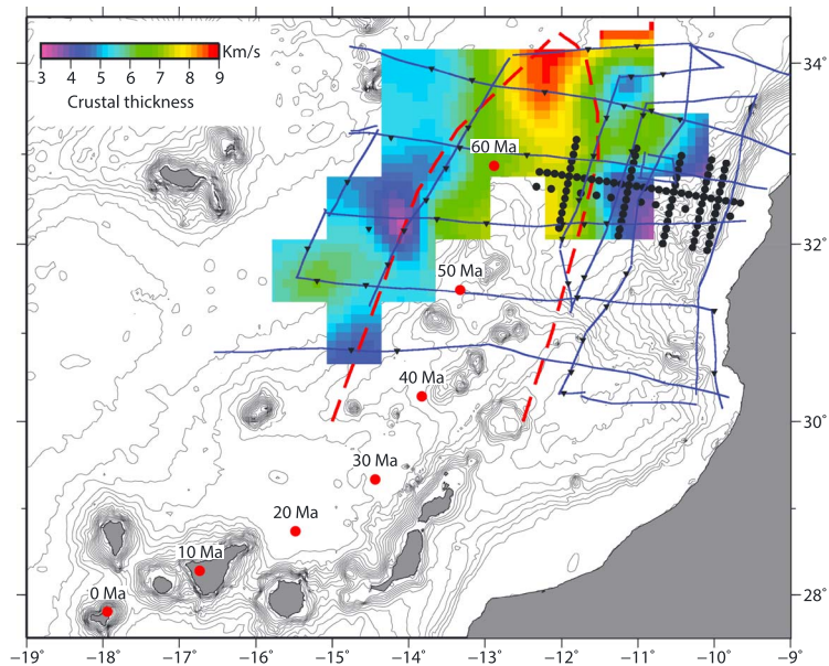
Figure 15. Lower crustal thickness in the southern segment from sonobuoy and ocean bottom seismometer (OBS) deployments [Holik et al., 1991; Biari et al., 2015]. Background contoured bathymetry from satellite altimetry [Smith and Sandwell, 1997]. Positions of sonobuoys are marked by inverted triangles [Holik et al., 1991] and OBS [Biari et al., 2015] by black circles. Blue lines mark the position of multichannel seismic (MCS) profiles, the red dashed line marks the extent of the basement bulge from Holik et al. [1991], and red dots show the reconstructed position of the Canary hot spot over time [Carracedo et al., 1998].
