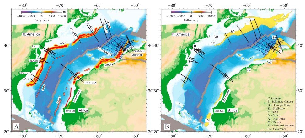
Figure 2. Reconstruction of the central Atlantic at M25 pole from Seton et al. [2012]. Locations of wide-angle seismic profiles are marked by black lines. (a) Location of the magnetic anomalies ECMA = East Coast Magnetic Anomaly; WACMA = West African Coast Magnetic Anomaly, BSMA = Blake Spur Magnetic Anomaly, and ABSMA = African Blake Spur Magnetic Anomaly. (b) Location of the main salt basins shown in yellow.
