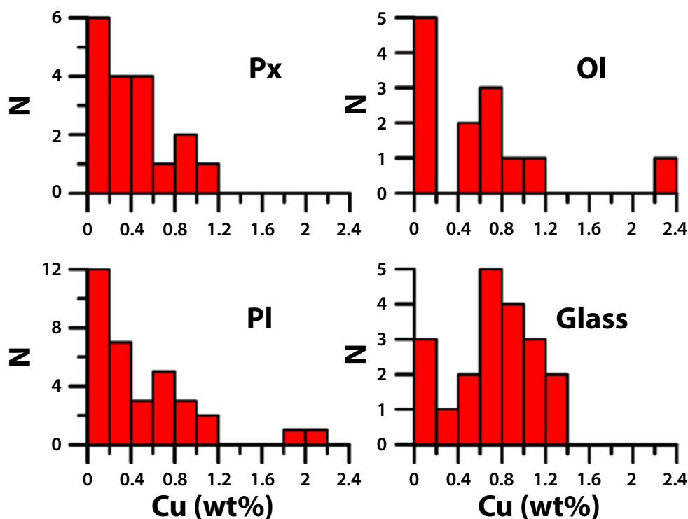
Fig. 5. Cu concentrations in pyroxene (Px), olivine (Ol), and plagioclase (Pl) grains from shocked unmelted basaltic clasts in agglutinate-like particles and in heterogeneous glasses. N is the number of analyses.
