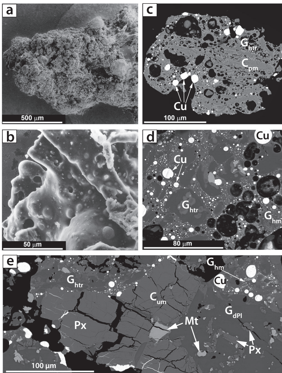
Fig. 2. a) Secondary electron (SE) image of agglutinate-like particle (shot 19, see Table 1). The particle surface is covered by strongly adhered basaltic dust. b) SE image of agglutinate-like particle surface details (shot 9); the surface is partially covered by a glass film; numerous knobs are copper droplets in the glass. c) Backscatter electron (BSE) image of the section of particle 9-s3 from shot 9 (see Table 1). The particle is composed of partially melted basaltic clasts ( C_{pm} ; the clasts are composed of a plagioclase melt glass and both melted and unmelted pyroxene) in a porous glassy matrix with disseminated copper droplets (white); partially melted clasts preserved in some parts the original texture; heterogeneous glass ( G_{htr} ) is present. d) BSE image of a fragment of agglutinate-like particle 26-s3 from shot 26 (Table 1). Inclusions of the heterogeneous glass (dark gray areas of different gradation with no white copper droplets) are embedded in the homogeneous glass ( G_{hm} ) with numerous copper droplets (Cu). e) Mosaic image of a fragment of particle 18-2 (shot 18) consisting of an unmelted basaltic clast ( C_{um} ) in heterogeneous and homogeneous glasses. The clast is composed of pyroxene (Px), plagioclase diaplectic glass ( G_{dPl} ), and magnetite (Mt).
