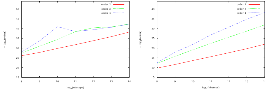
Fig. 4. Experimental evaluation of the order of the IDE numerical integrator over Volterra-Kostitzin model (1), with an integral lower bound equal to zero. On the left hand picture, the kernel is a cubic spline (i.e. a C^2 curve). On the right hand picture, the kernel is a smooth curve (on the two pictures, the mathematical problem to be solved is thus not the same). In each picture, there is one curve per Butcher tableau of Fig. 3. Each curve was obtained as follows: a first integration was performed with 2^{15} steps. Its result was then considered as a reference value and compared with the result of other integrations with 2^8, 2^9, \dots, 2^{14} steps, giving 7 points hence a curve, which should be a straight line (see formula (11)). Its slope is a numerical estimate of the order of the numerical integrator. In the case of a C^2 kernel, the integrator has order 2 when used with an order 2 tableau; and a non reliable order when used with order 3 and 4 tableaux. In the case of a smooth kernel, the integrator has the same order as the tableau with which it is used (the curve for order 4 is slightly irregular because the order of the quadrature formula does not match the one of the Butcher tableau).
