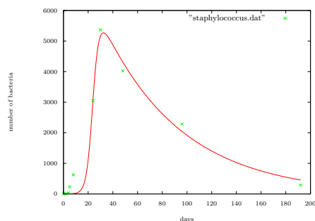
Fig. 5. Best fitting curve for (1) with a trivial kernel and an integral lower bound equal to zero, against the staphylococcus population reported in [23, page 72]. Optimal parameters are \varepsilon = 3.97 \times 10^{-1} , \lambda = 6.56 \times 10^{-5} and \mu = 1.02 \times 10^{-6} .
