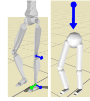
Figure 1: left : joints affected by the ground contact stabilizer, right : example of reduced model where all the body parts above the pelvis have been simplified by a single force
