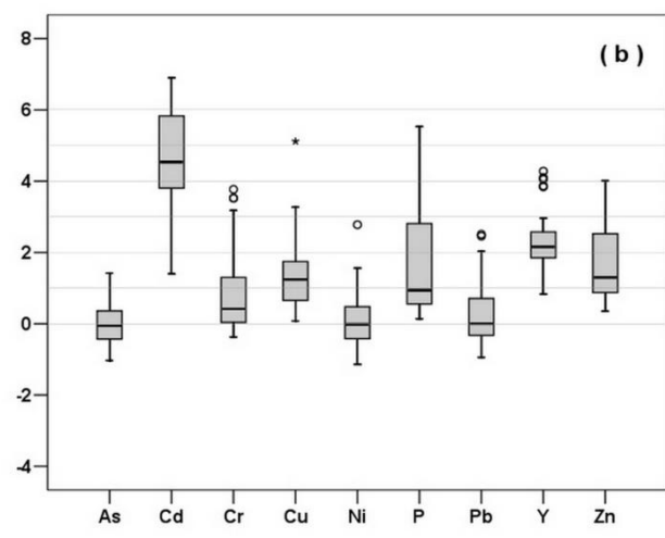
Fig.4 Box-and-whisker plots for enrichment factors (a) and geoaccumulation index(b) of heavy metals in the surface sediments.
