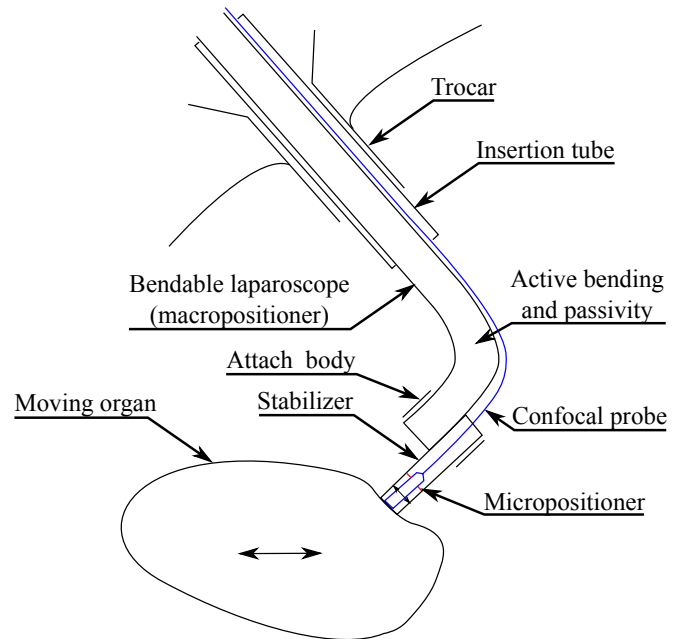
Fig. 2. Schematic view of the system. Note that the active bending is realized with external motors and cables
