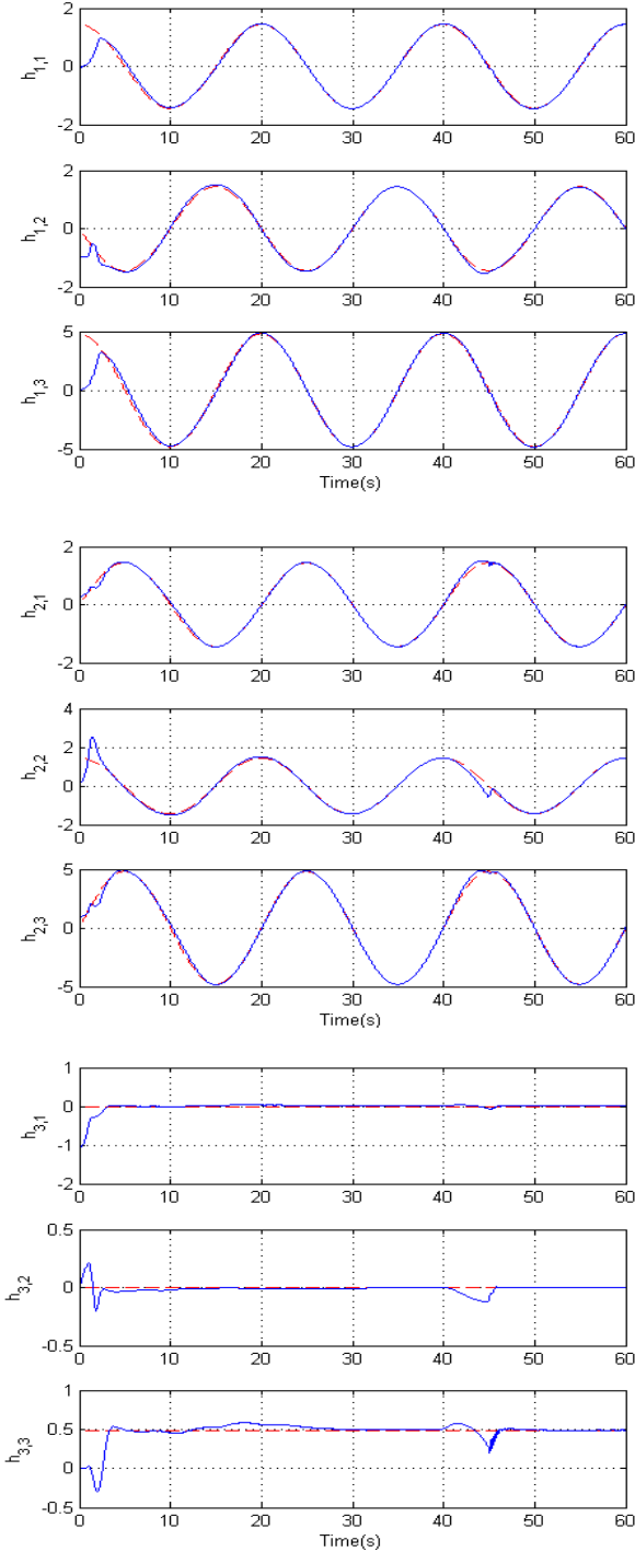
Fig. 1. Estimated homography components (solid line) and true homography ones (dashed line) vs. time.
