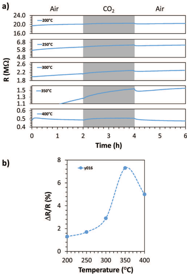
Fig. 6. For the y016 sample: a) resistance in the presence of air ( R_{\text{air}} ) and CO 2 ( R_{\text{CO}_2} ) in the 200–400 °C temperature range and b) \Delta R/R_{\text{air}} with at various operating temperature.
