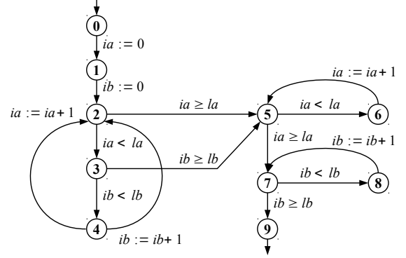
Figure 4: Simplified LTS for the merging sort example.
