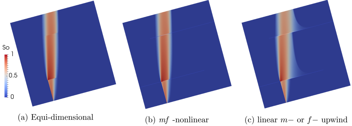
Figure 4: Oil saturation at final time computed by the equi-dimensional and hybrid-dimensional models for the gravity dominant test case with homogeneous capillary pressures. The mesh is Cartesian of size 260 \times 264 for the equi-dimensional model and of size 256 \times 256 for the hybrid-dimensional models.
