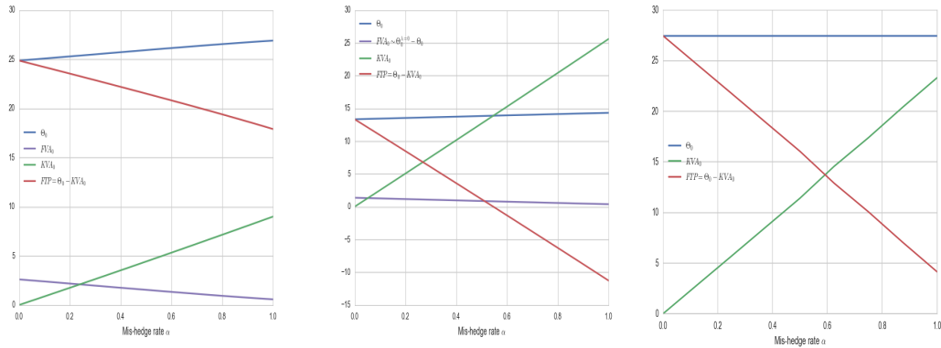
Figure 1: XVAs and FTP as a function of the mis-hedge parameter \alpha . Left : Without model uncertainty. Middle : With UVM uncertainty ( \underline{\sigma} = 15\% , \bar{\sigma} = 60\% ). Right : With OT uncertainty ( \underline{\sigma} = 15\% , \bar{\sigma} = 60\% , \sigma = 30\% ).
