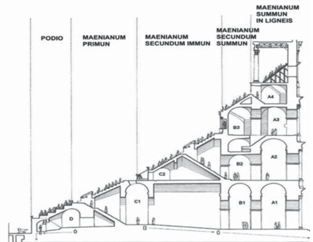
Fig. 3: The different levels in the Colosseum.
