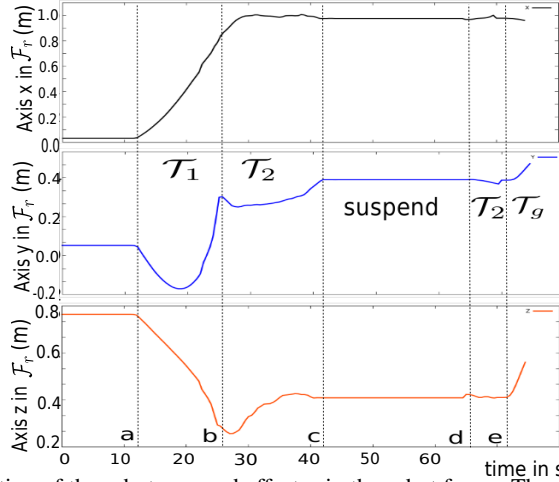
Fig. 13: Real position of the robot arm end effector in the robot frame. The motion starts at time a ; Between a and b : the controller tracks the first trajectory segment \mathcal{T}_1 in \mathcal{F}_r ; From b to c and d to e : target tracking; From c to d : the task is suspended; From e to end: the grasping movement controlled in \mathcal{F}_o .
