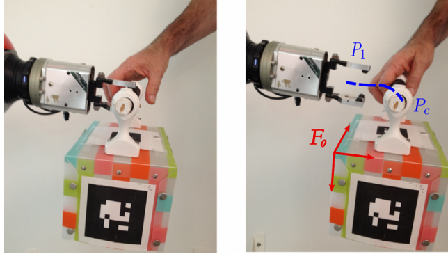
Fig. 5: A simple case of grasp. Left: a planned grasp defines contact points between the end effector and the object. Right: To finish the grasping, the manipulator must follow the blue trajectory P_1 - P_c , and then close the gripper. This movement must be controlled in the object frame F_o .
