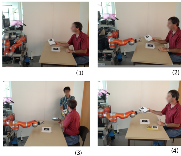
Fig. 12: (1): The controller is given the task of receiving the object from human. It tracks the first segment in the robot frame. (2): The object is moving and the robot tracks a target. (3): Human is distracted by another human and the task is suspended. (4): Human returns to the task, and the robot resumes the task and grasps the object.
