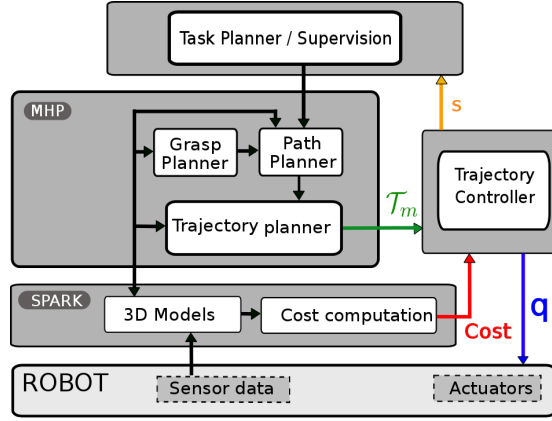
Fig. 1: Software Architecture of the robot for HRI manipulation. \mathcal{T}_m is the main trajectory calculated initially by MHP (Motion in Human Presence). The controller takes also cost maps from SPARK. The controller sends control signals in joint ( q in the figure) to the servo system, and during the execution, the controller sends the state of the controller ( s ) to the supervisor
