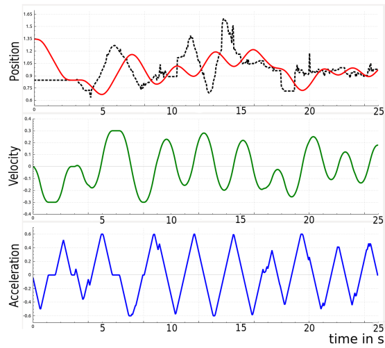
Fig. 11: Results of robot tracking a target: position (in m ), velocity (in m/s ) and acceleration (in m/s^2 ) during the tracking for 25 seconds. The black dashed line is the target position, with noise of the 3D vision, and the red line is the position of the robot, which tracks the target with a delay. The positions of the robot are calculated from measured joint values and the kinematic model, while velocity and acceleration are estimated. The velocity, acceleration and jerk are always limited, maintaining a smooth tracking process.
