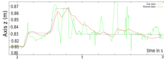
Fig. 10: Instability of the 3D vision in poor lighting condition. The green curve shows axis z of the localization result of an object in the robot frame over 10 seconds and the red one shows the filtered result. The object was held by a human that intended to move the object accordingly to the black dashed curve.
