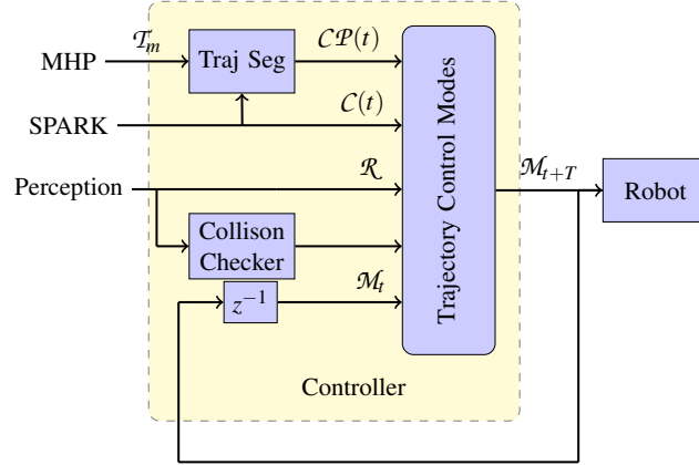
Fig. 4: Input and output of the controller. \mathcal{T}_m is the trajectory computed by MHP, it is then segmented into control primitives ( C\mathcal{P}(t) ). Traj Seg represents trajectory segmentation . C(t) are the cost values. \mathcal{R} represents the transformation matrices, giving the position of the target and of the robot. \mathcal{M}_t is the current state of the robot, \mathcal{M}_{t+T} is desired motion condition for the next control cycle. z^{-1} represents delay of a control cycle.
