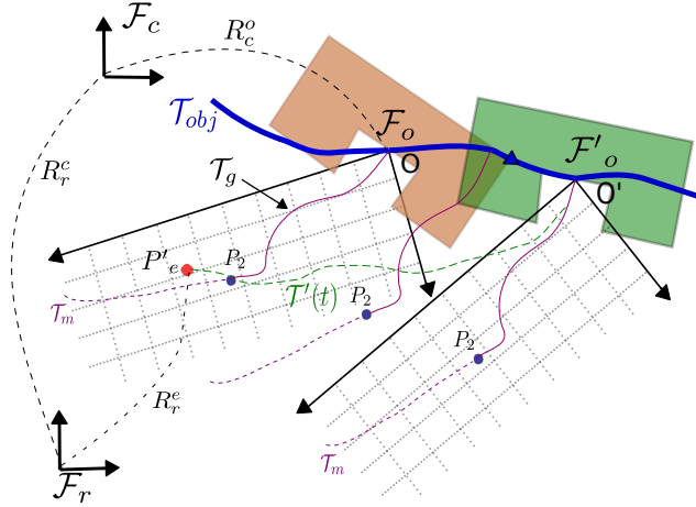
Fig. 9: Control Mode 2 . control mode. Object at time t_1 is colored in light brown, and green at time t_2 . It follows a movement model given as the blue trajectory \mathcal{T}_{obj} . The purple trajectory for grasping \mathcal{T}_g stays unchanged in the object frame. The robot tracks the trajectory \mathcal{T}'_g as it does the grasping movement.
