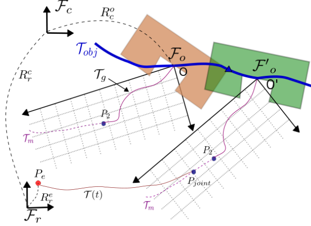
Fig. 8: Control Mode 1 . The robot tracks a point. The object moves to the right, it is drawn at two times: firstly in brown for time t_1 and then in green at time t_2 . In both cases, the entry point P_2 of the trajectory \mathcal{T}_g is drawn relatively to the object frame \mathcal{F}_o .
