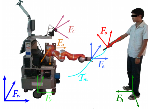
Fig. 2: Frames for object exchange manipulation: F_w : world frame; F_r : robot frame; F_c : camera frame; F_e : end effector frame; F_o : object frame; F_h : human frame. The trajectory realizing a manipulation should be controlled in different task frames.
