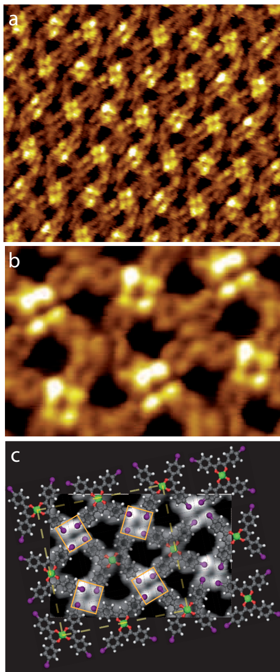
Figure 3: High resolution STM images of the complex-1 self-assembled porous network, (a) 10 \times 8 \text{ nm}^2 , V_s = 0.95 \text{ V} , I_t = 9 \text{ pA} , (b) 5 \times 3 \text{ nm}^2 , V_s = 0.95 \text{ V} , I_t = 9 \text{ pA} . (c) Assembly model with the STM image in (b) placed underneath as a guide for the eyes. X 4 synthons are highlighted with orange squares.
