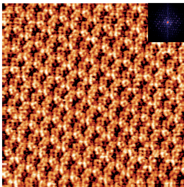
46 47 48 49 50 51 52 53 54 55 56 57 58 59 60 Figure 4: STM image of the complex-2 self-assembled porous network at the 1-phenyloctane/graphite interface, 27 \times 27 nm 2 , V_s = 0.95 V, I_t = 9 pA. Inset: FFT of the STM image.
