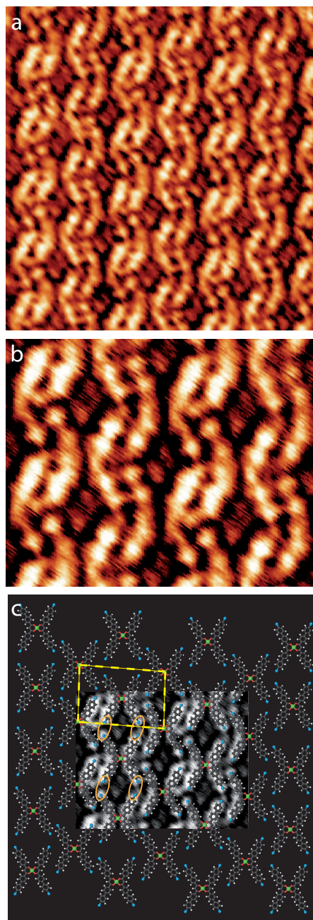
Figure 5: High resolution STM images of the complex-2 self-assembled porous network, (a) 15 \times 15 \text{ nm}^2 , V_s = 0.95 \text{ V} , I_t = 9 \text{ pA} , (b) 8 \times 6 \text{ nm}^2 , V_s = 0.95 \text{ V} , I_t = 9 \text{ pA} . (c) Assembly model with the STM image in (b) placed underneath as a guide for the eyes. X 2 synthons are highlighted with orange ellipses.
