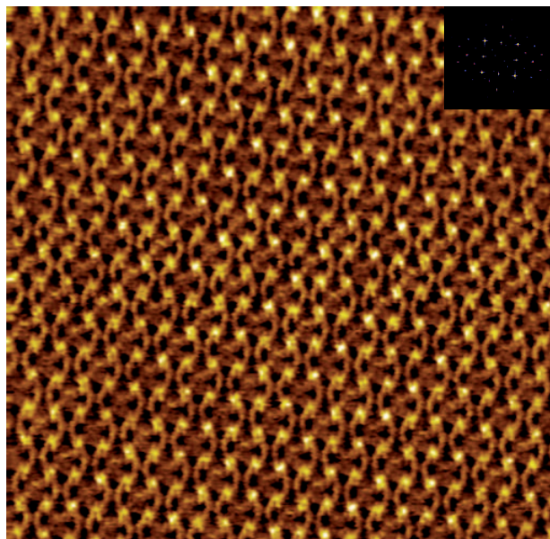
Figure 2: STM image of the complex-1 self-assembled porous network at the 1-phenyloctane/graphite interface, 35 \times 35 \text{ nm}^2 , V_s = 0.55 \text{ V} , I_t = 9 \text{ pA} . Inset: FFT of the STM image.
