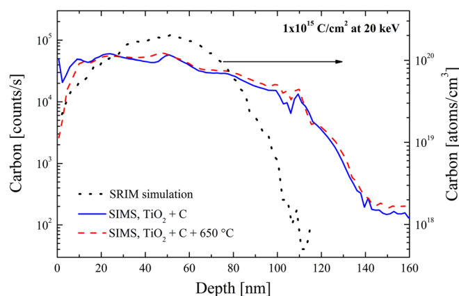
FIG. 1. Carbon chemical profiles just after the implantation ( 1 \times 10^{15} \text{ cm}^{-2} at 20 keV, straight line) and after annealing at 650^\circ\text{C} for 2 h (dashed line). The simulation 26 of the implanted profile is also reported on the right vertical axis (dotted line).
