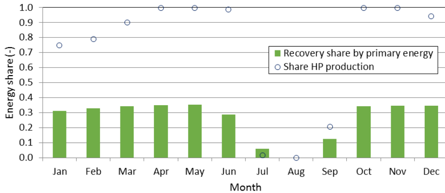
Figure 4. District heating with sewage water heat recovery performance data from on-site monitoring
