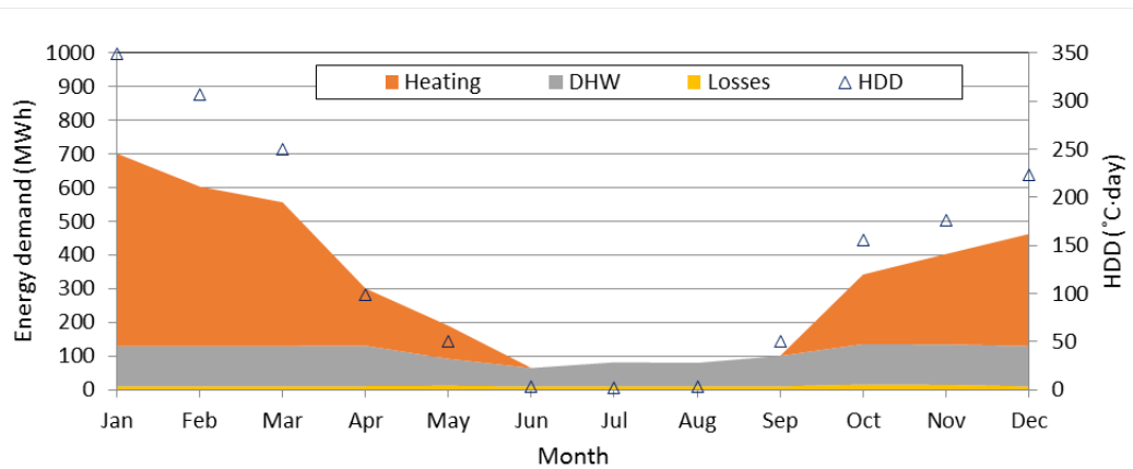
a) Energy demand from central heating, DHW and heat losses
