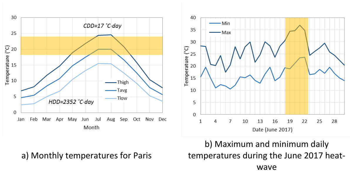
Figure 1. Air temperature data at the Montsouris weather station in Paris
