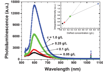
Fig. 2. Photoluminescence spectra of DsRed dehydrated droplets adsorbed on SiO 2 surface for different concentrations at pH = 7.0 and 23°C. The inset represents the integrated intensity of the photoluminescence peak as a function of the DsRed concentration.
