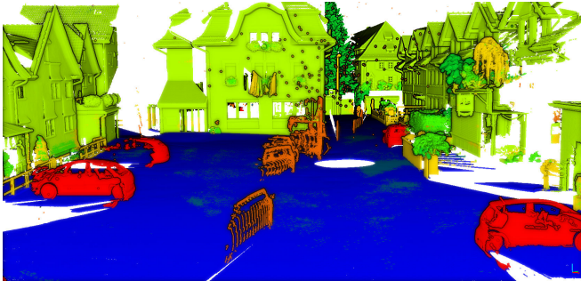
Fig. 3. Example of classified point cloud on Semantic3D test set (blue: man-made terrain, cerulean blue: natural terrain, green: high vegetation, light green: low vegetation, chartreuse green: buildings, yellow: hard scape, orange: scanning artefacts, red: cars).
