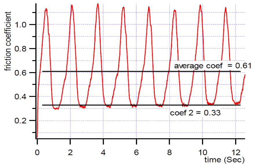
Figure 11 : Evolution of the ply/ply friction coefficient for the G1151® interlock fabric
