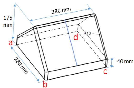
Figure 1 : Punch dimensions
