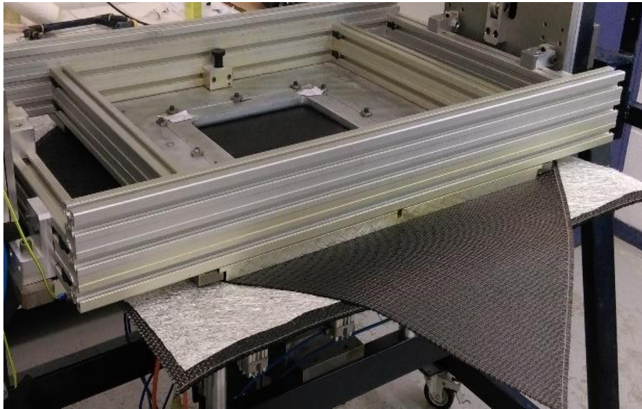
Figure 14 : Configuration of two layer preforming (45°/0°) with mat inserting.
