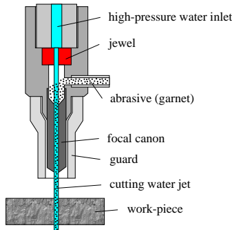
Fig. 1. Schematic drawing of the AWJ process.
