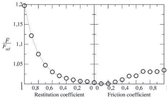
Fig. 3. Relative evolution of the AWJ reaction on plane according to contact parameters: energy restitution and friction coefficient.
