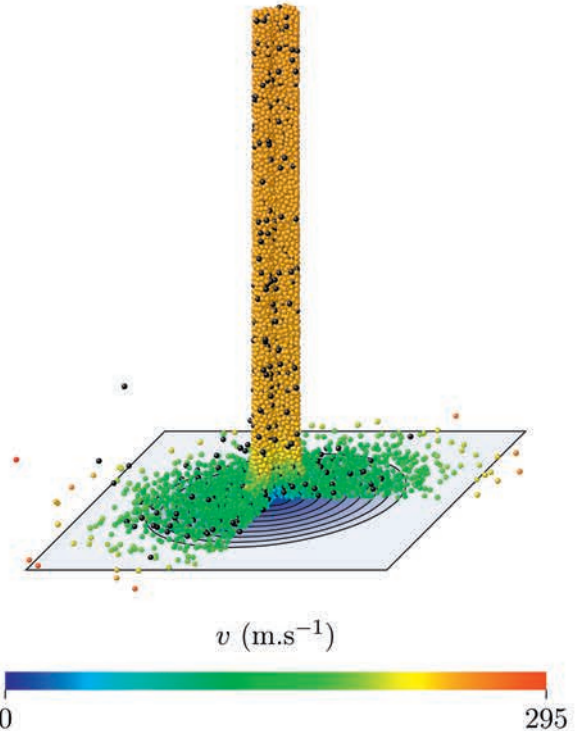
Fig. 4. Example of \frac{3}{4} of AWJ granular medium and its velocity field simulated just after impact, with 10 mm of canon/work-piece distance and 5 % of volumic ratio of abrasive particles. These last ones are drawn in black.
