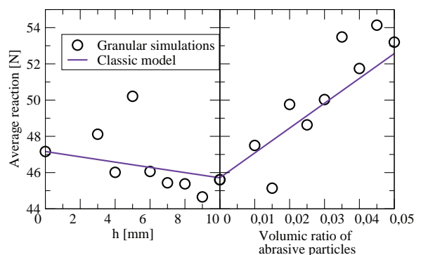
Fig. 7. Evolution of the AWJ reaction according to process parameters: canon/work-piece height h and volumic ratio of abrasive particles. Data from granular simulations are compared to the predictive model.
