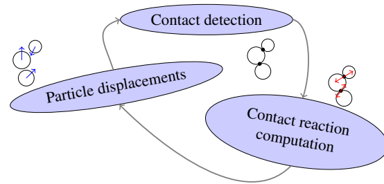
Fig. 2. Algorithm pattern of a single iteration of discrete element method.
