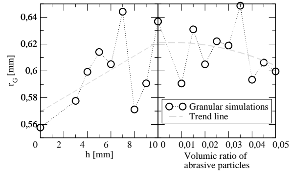
Fig. 8. Evolution of the Gaussian fit influence radius according to process parameters: canon/work-piece height h and volumic ratio of abrasive particles. These data are extracted from granular simulations and the trend lines are plotted.
