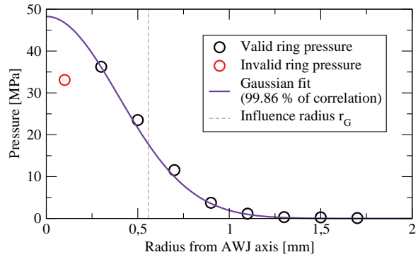
Fig. 6. Simulation values & Gaussian fit of a pure water-jet pressure split on several concentric rings, without air dissipation phenomenon.
