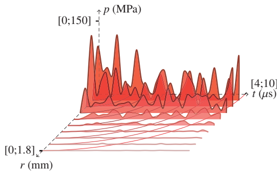
Fig. 5. Evolution of a pure water-jet pressure split on several concentric rings, according to time. This simulation does not take into account air dissipation phenomenon.
