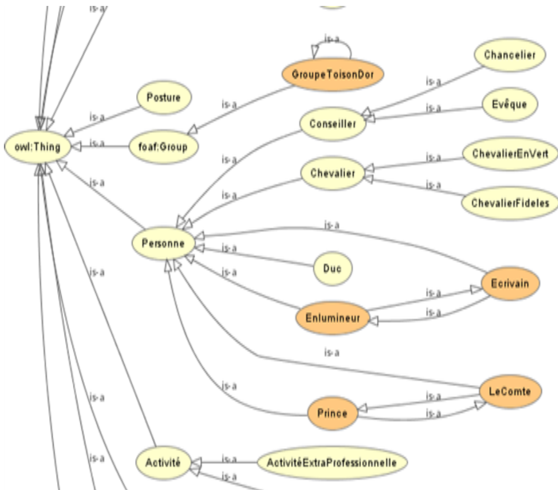
Figure 2: A view in Protege 2000 of some concepts of illumination of figure 1. These concepts are organised through the subsumption relation ( is - a ).
