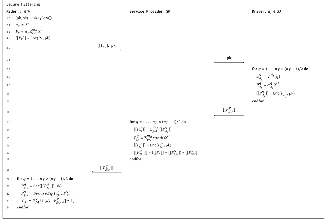
Figure 3: Secure filtering protocol.
