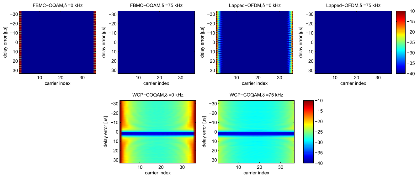
FIGURE 9. WFs with real orthogonality: per-subcarrier NMSE against TO, \delta = 0 and 75kHz.
