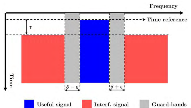
FIGURE 2. Coexistence scenario: two asynchronous users with \tau [s] TO, \epsilon [kHz] CFO and free guard-bands of \delta [kHz].
