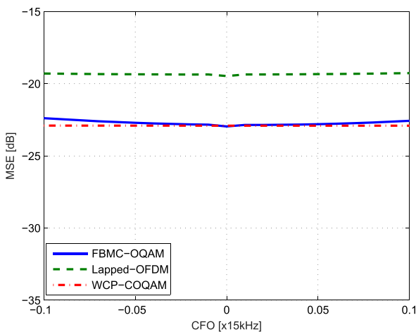
FIGURE 16. WFs with real orthogonality: average MSE against CFO, \delta = 0\text{kHz} .
