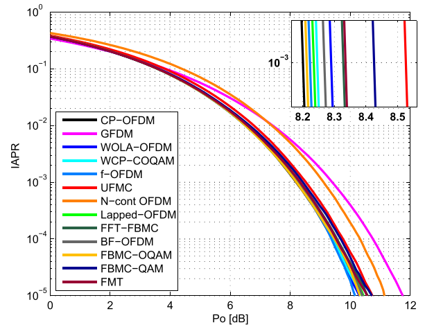
FIGURE 19. (Comparison of the CCDF of the IAPR.
