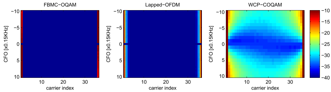
FIGURE 15. WFs with real orthogonality: per-subcarrier NMSE against CFO, \delta = 0\text{kHz} .
