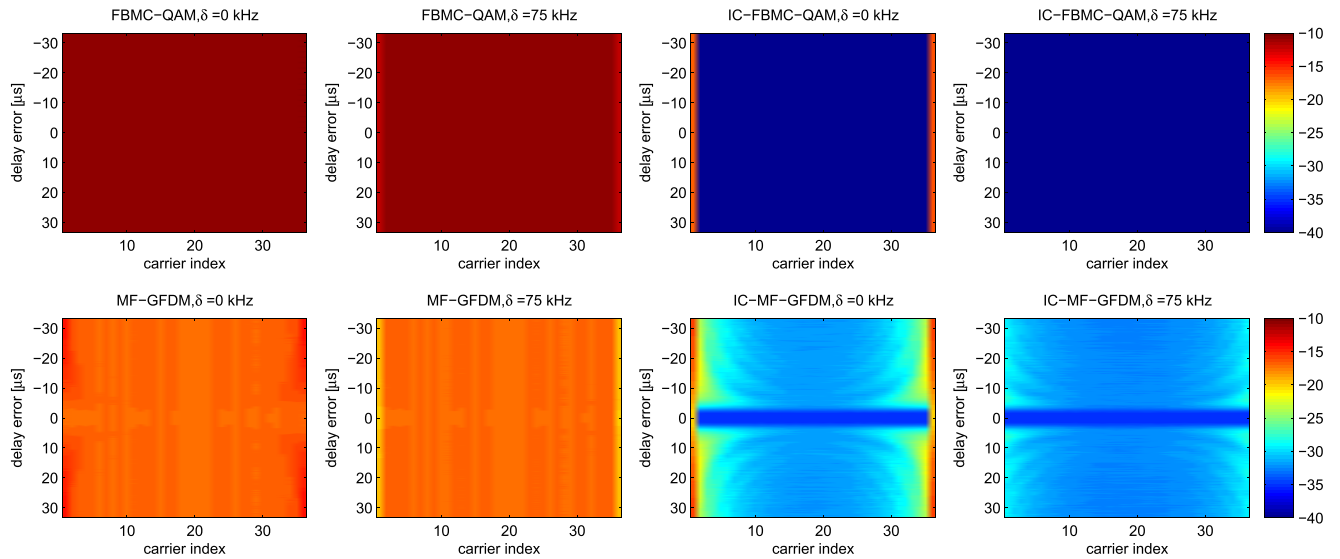
FIGURE 11. Non-orthogonal WFs without and with interference cancellation (IC): per-subcarrier NMSE against TO, \delta = 0 and 75kHz.
