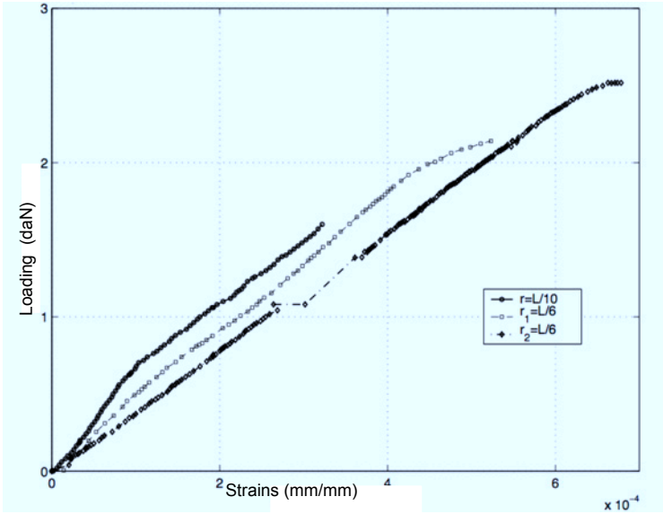
Figure 12. Compression diagonal test - Strain of compressive diagonal
