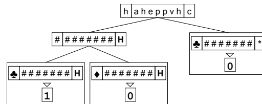
Figure 10: anticipation tree for hearing; the only action that provokes sound is hitting, it is true only if the object is food or the agent is hungry; when the agent hits (H) an object that is food or a non-aggressive agent, differentiated of their confounding pairs by the synthetic element (♣), then the agent listens a sound in the next instant; if the action is other (*) than hitting, then no sound is produced.
