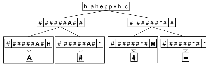
Figure 11: anticipation tree for vision; when the agent hits (H) another agent (A), it verifies the permanence of this other agent in its visual field, which means that hitting an agent makes it stay in the same place; however, no other actions (*) executed in front of an agent (A) can prevents it to go, and so the prediction is undefined (#); the same for moving itself (M), which causes a situation changing and the non predictability of the visual field for the next instant; in all of the other cases the vision stays unchanged.
