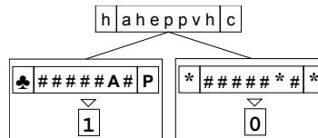
Figure 12: anticipation tree for pain; the agent knows that playing (P) with an aggressive (♣) agent (A) causes pain; otherwise, no pain is caused.
