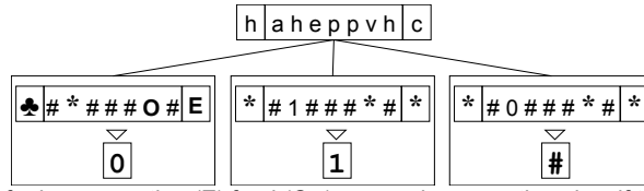
Figure 15: anticipation tree for hungry; eating (E) food (O♣) ceases hungry; otherwise, if the agent is already hungry, it will remains, but if it is not yet hungry, it can become.
