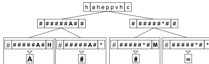
Figure 11: anticipation tree for vision; when the agent hits (H) another agent (A), it verifies the permanence of this other agent in its visual field, which means that hitting an agent makes it stay in the same place; however, no other actions (*) executed in front of an agent (A) can prevents it to go, and so the prediction is undefined (#); the same for moving itself (M), which causes a situation changing and the non predictability of the visual field for the next instant; in all of the other cases the vision stays unchanged.
