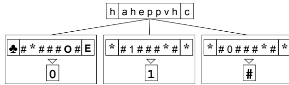
Figure 15: anticipation tree for hungry; eating (E) food (O♣) ceases hungry; otherwise, if the agent is already hungry, it will remain, but if it is not yet hungry, it can become.
