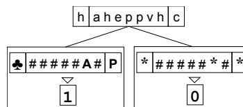
Figure 12: anticipation tree for pain; the agent knows that playing (P) with an aggressive (♣) agent (A) causes pain; otherwise, no pain is caused.
