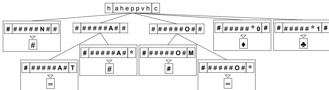
Figure 17: hidden element anticipation tree; this element allows identifying whether an object is food or stone, and whether an agent is angry or not; CALM abstract anticipation method allows modeling the dynamics of this variable, even if it is not directly observable by direct sensory perception; the perception of the noise (1) is the result that enables the discovering of the value of this hidden property; the visual perception of an object (O), or the fact of hitting (H) another agent (A), also permit to know that the hidden element does not change.
