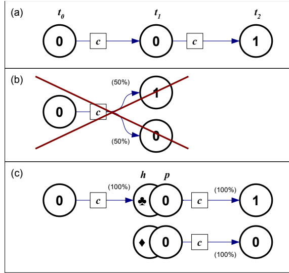
Figure 6: discovering the existence of non observable properties; in (a) a real experienced sequence; in (b) what CALM does not do (the attribution of a probability); in (c) the creation of a synthetic element in order to explain the observed difference.
