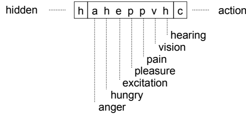
Figure 9: the vectors that compose the context of a schema; synthetic properties, perceptive properties, and controllable properties (actions).
