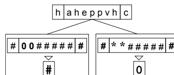
Figure 13: anticipation tree for pleasure; playing with a peaceable (♦) agent (A) is pleasant, and it is the only known way to reach this feeling.
