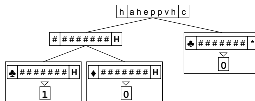
Figure 10: anticipation tree for hearing; the only action that provokes sound is hitting, it is true only if the object is food or the agent is hungry; when the agent hits (H) an object that is food or a non-aggressive agent, differentiated of their confounding pairs by the synthetic element (♣), then the agent listens a sound in the next instant; if the action is other (*) than hitting, then no sound is produced.
