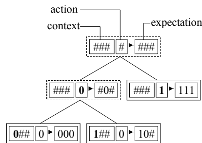
Figure 1: the anticipation tree; each node is a schema composed of three vectors: context, action and expectation; the leaf nodes are decider schemas.
