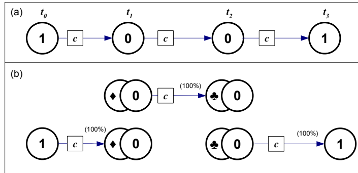
Figure 7: predicting the dynamics of a non observable property; in (a) a real experienced sequence; in (b) the pieces of knowledge that can explain the logic behind the observed transformations, including the synthetic property changing.
