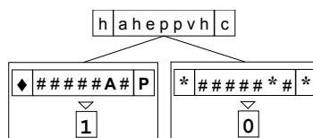
Figure 13: anticipation tree for pleasure; playing with a peaceable (♦) agent (A) is pleasant, and it is the only known way to reach this feeling.
