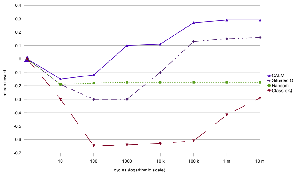
Figure 18: the evolution of mean reward in a typical execution of the meph problem, considering four different agent solutions: CALM, situated Q-Learning, Random, and Classic Q-Learning; the scenario is a 25x25 grid, where 10% of the cells are stones and 5% are food, in the presence of 10 other agents.
