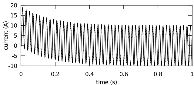
(b) MECSYCO simulation results.
