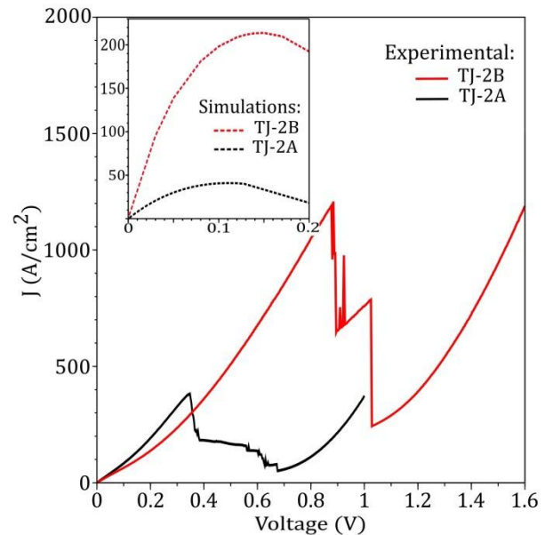
Fig. 5: Experimental J-V characteristics of samples without (TJ-2A in black) and with (TJ-2B in red) the inclusion of the GaAsSb/InGaAs QW. The simulation results are presented in the inset, with the black dashed curve for TJ-2A and the red dashed curve for TJ-2B.
