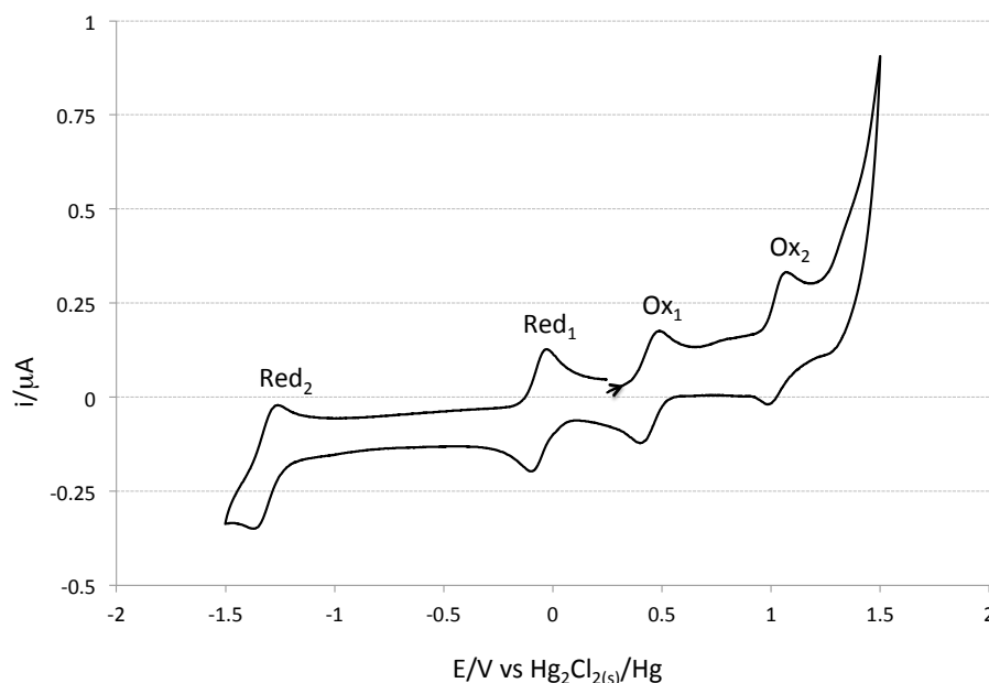
Fig. 5. Cyclic voltammogram of 1 carried out at a scan rate of 100 \text{ mV}\cdot\text{s}^{-1} in dichloromethane containing 0.1\text{M Bu}_4\text{NPF}_6 as supporting electrolyte. Potentials were measured vs. SCE using a Pt working electrode. Waves Red 1 and Ox 1 were reversible, and waves Red 2 and Ox 2 were quasi-reversible.
