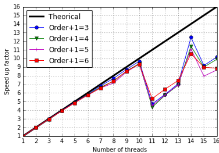
Figure 7. Scalability of the SSE4.2 code.
