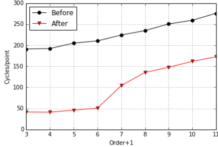
Figure 3. Cpp by approximation order+1 comparing a scalar mono-thread execution using a IVB processor.
