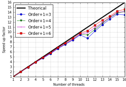
Figure 5. Scalability of the new code.
