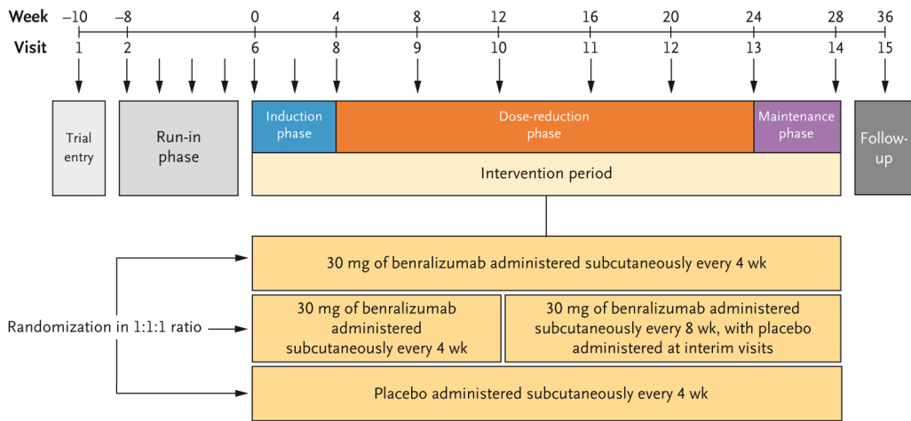
Figure 1. Trial Design.
