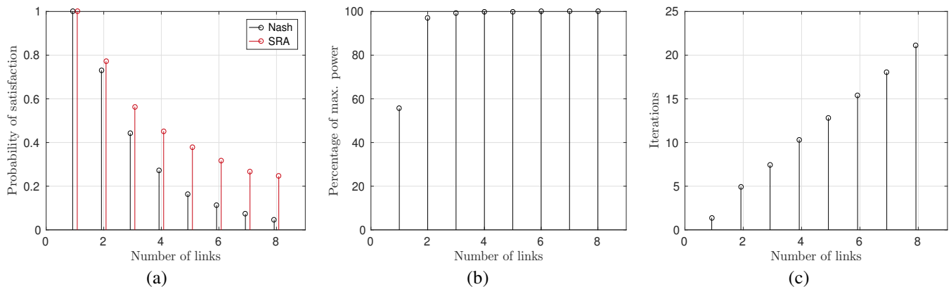
Fig. 3. DSSS game with 1-bit feedback and Algorithm 2, \Gamma_i^{(\text{dB})} = 15 dB, \forall i \in I . From left to right: probability of satisfaction, average power used by satisfied players, average number of iterations to a GSE.
