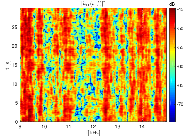
Fig. 1. A channel frequency response from the UWA channel simulator from [42], [43].
