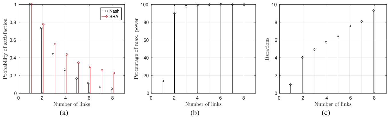
Fig. 2. DSSS game with SINR feedback and Algorithm 1, \Gamma_i^{(\text{dB})} = 15 dB, \forall i \in I . From left to right: probability of satisfaction, average power used by satisfied players, average number of iterations to a GSE.
