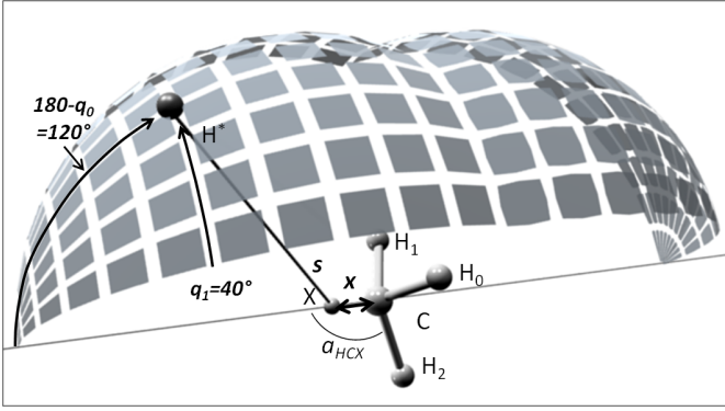
FIG. 8. Illustration of a typical bi-faceted dividing surface of the \text{CH}_3+\text{H}\rightarrow\text{CH}_4 reaction.
