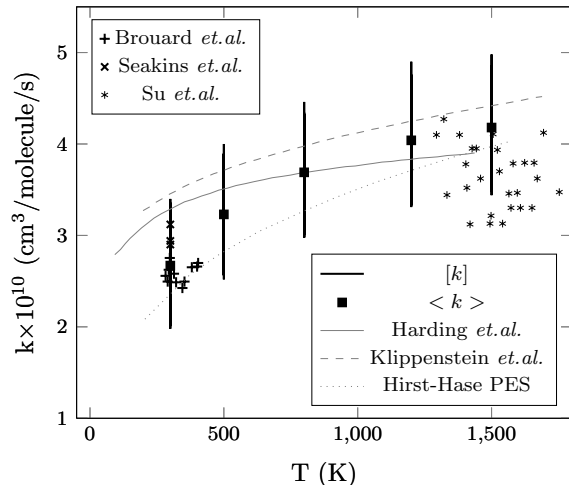
FIG. 12. Comparison of the high pressure \text{CH}_3+\text{H} recombination rate predicted by this work (black lines: [k] , squares: \langle k \rangle ) with other theoretical calculations (gray lines) and the experimental values (crosses 66 , asterisks 67 , times 65 ). Gray lines: calculations using different representation of the PES; full line: on the fly calculation 17 , dashed line: 4D mathematical fit 16 , dotted line Hirst-Hase PES.
