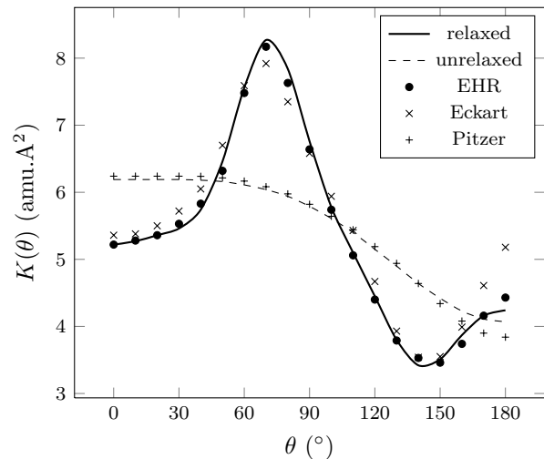
FIG. 3. Comparison between the kinetic function calculated in this work (lines) and the kinetic function obtained using the Extended Hindered Rotor model 11 (EHR), the Eckart method 9 and the Pitzer method 57 (presented by Wong et al. 9 ). Solid line: flexible torsion ( f_i(\theta) \neq 0 ); dashed line: rigid rotation ( f_i(\theta) = 0 ).
