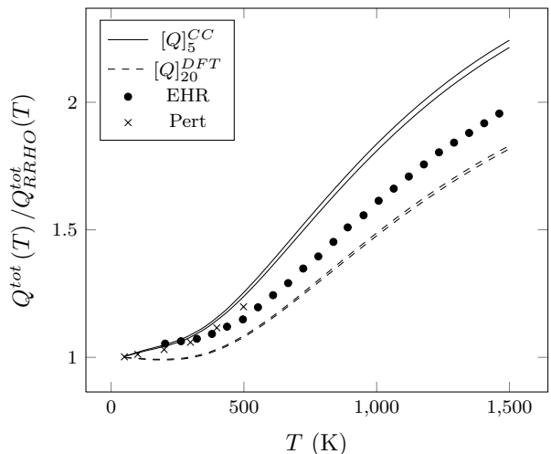
FIG. 7. Comparison between the 95% confidence interval of the posterior partition function of the butadiene using D_{20}^{DFT} (dashed line) and D_5^{CC} (solid line, \sigma_M^2 = 1.25 \cdot 10^{-3} ). Crosses: Pert method 58 , circles: EHR method 11 . Results normalized to the RRHO partition function.
