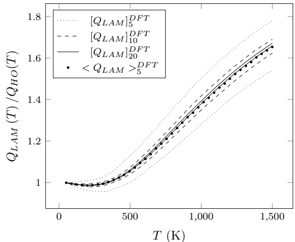
FIG. 6. 95% CI of the posterior torsional partition function using the data set D_n^{DFT} with n = 5 (dotted line), n = 10 (dashed line) and n = 20 (solid line). Filled circles: mean of the posterior torsional partition function using D_5^{DFT} . Results are normalized by the HO partition function.
