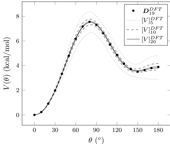
FIG. 4. 95% confidence interval of the posterior PES using the data set \mathbf{D}_n^{DFT} with n = 5 (dotted line), n = 10 (dashed line) and n = 20 (solid line). Filled circles represent the data set \mathbf{D}_{19}^{DFT} .
