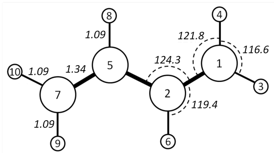
FIG. 2. Illustration of the geometry of 1,3-butadiene at the global minimum of the PES. The large circles represent the carbon atoms, and the small circles represent the hydrogen atoms. Bond lengths are in Angstroms and angles in degrees. The atom numbering used in the paper are indicated in the circles.
