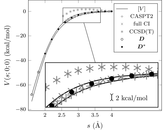
FIG. 10. Comparison between the predicted 95% confidence interval of the MEP ( [V] ), the datasets \mathbf{D} and \mathbf{D}^* and the ab initio results presented in literature. Lines: [V] ; black circles: \mathbf{D}^* , empty circles: \mathbf{D} . Grey symbols: literature results; asterisks: CCSD(T)/6-31G(d) 17 , crosses: CASPT2/aug-ccVQZ 17 , times: full CI/6-31G(d) 64 . Origin of energy: V(4 \text{ \AA}, 0, 0) .
