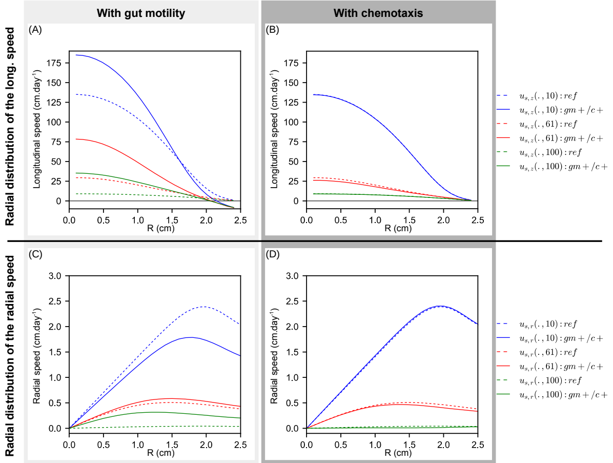
Figure Appendix B.5: Radial distribution of the longitudinal and radial speeds at z = 10 , 61 , and 100\text{cm} . To assess the effect of peristalsis and chemotaxis on the spatial structure of intestinal hydrodynamics, we display the radial distribution of the speed components at z = 10 , 61 , and 100\text{cm} with gut motility ( gm+ , A and C) or bacterial chemotaxis ( c+ , B and D), compared with the reference of Fig. 3 ( ref , dashed lines). When the gut motility is active, negative speeds near the wall are observed, inducing a large increase of the longitudinal speed in the luminal part (blue line, A). Namely, if some material is transported upstream in the wall vicinity, as no outflux is possible in the proximal gut, a higher speed must be applied in the lumen to evacuate this additional material income in order to prevent volume expansion in the proximal gut. The difference of order of magnitude between the small upstream speed near the mucosa and the large downstream speed at r = 0 is due to the cylindrical geometry. In cylindrical coordinates, the elementary volumes near the wall are larger than the luminal ones. Hence, for a same transport speed, the amount of fluid transported in the epithelial vicinity is higher than in the lumen. Consequently, a higher speed must be applied near the gut axis to insure volume conservation.
