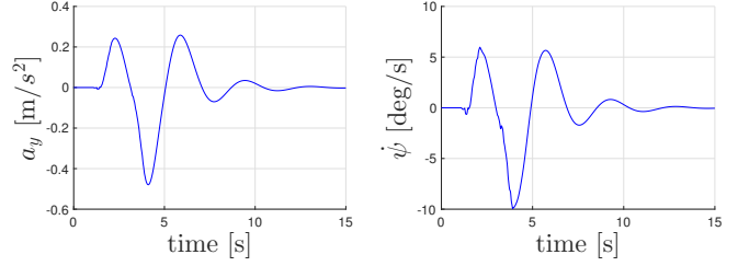
(a) Measured lateral acceleration
