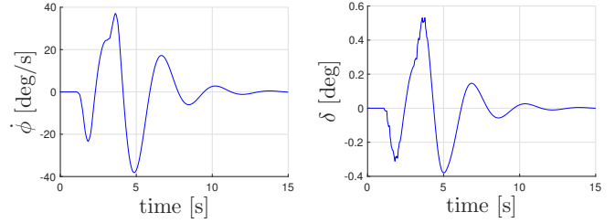
(c) Measured roll rate
