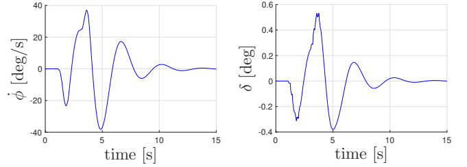
(c) Measured roll rate
