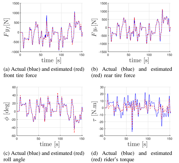
Fig. 6. Estimated states and unknown input
