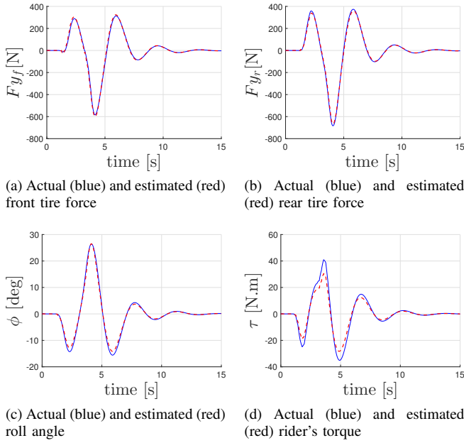
Fig. 3. Estimated states and unknown input
