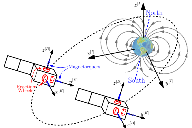
Fig. 1. An inertially pointing satellite orbiting around the earth and equipped with reaction wheels and magnetorquers.
