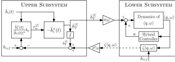
Fig. 2. The quasi-cascaded structure of the “cross product control law” and the role of the signal \zeta(q, \omega) .
