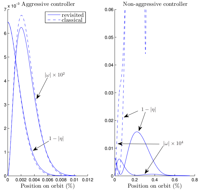
Fig. 3. Comparison in Remark 5 between the classical (dashed) and revisited (solid) “cross-product control laws” when using an aggressive attitude controllers (left-hand side plot) and a non-aggressive one (right-hand side plot).
