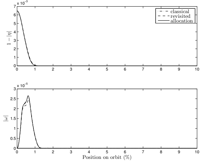
Fig. 6. Quaternion and \omega for the three approaches using an aggressive attitude controller.
