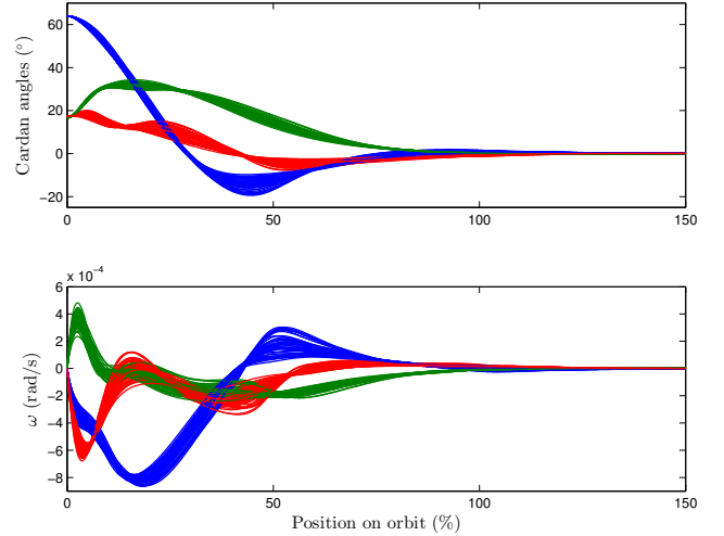
Fig. 10. Monte-Carlo study on uncertainties on J : Cardan angles and w for the revisited controller.
